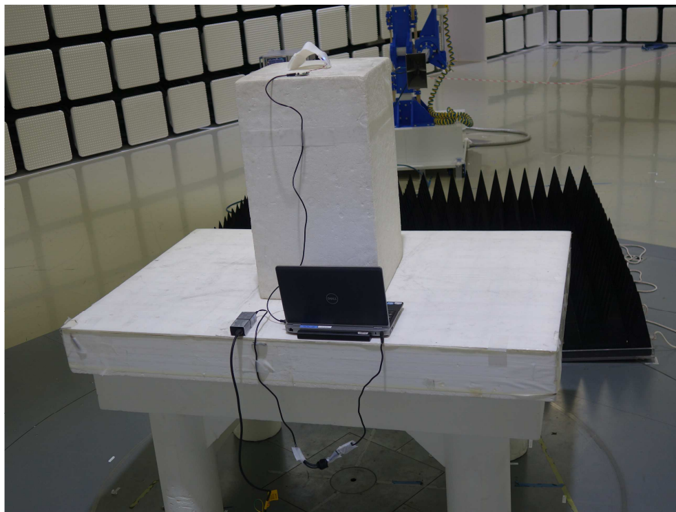
Photograph 5: Set-up for Radiated Emission of Transmitter at GHz Range, Rear View
