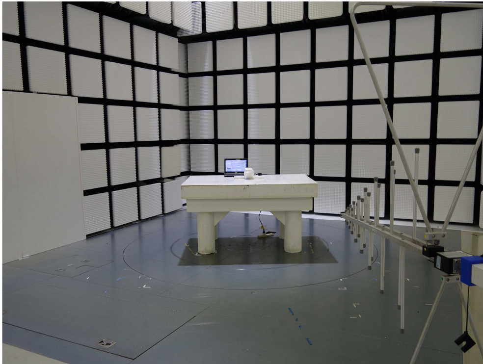
Photograph 2: Set-up for Radiated Emission of Transmitter at MHz Range, Front View
