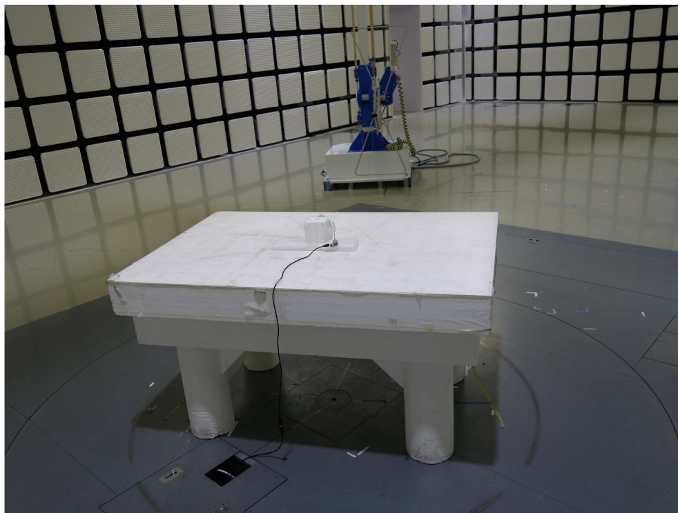
Photograph 3: Set-up for Radiated Emission of Transmitter at MHz Range, Rear View
