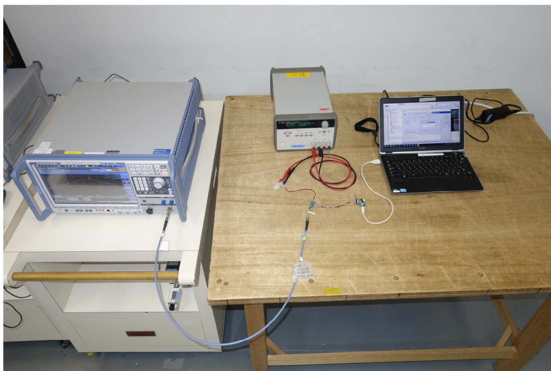
Photograph 6: Set-up for Antenna Port Connected Test
