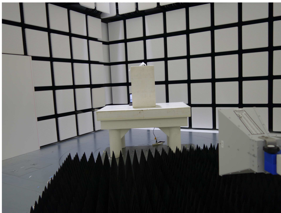
Photograph 4: Set-up for Radiated Emission of Transmitter at GHz Range, Front View
