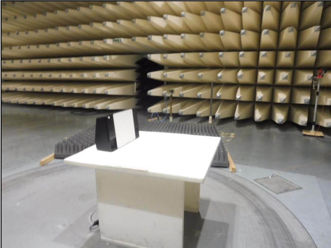
Photo 3: Test setup radiated emission
