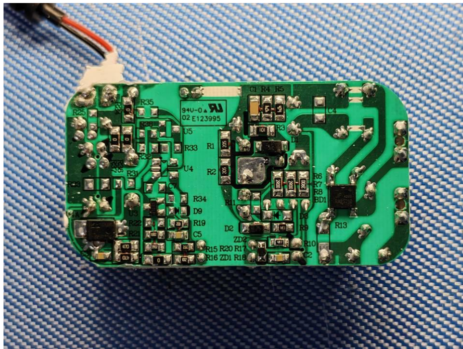
Picture 15_Adapter HCX2401-1202000U
