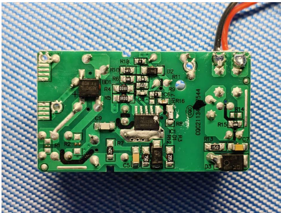
Picture 18_ Adapter GMB24-120200-1A
