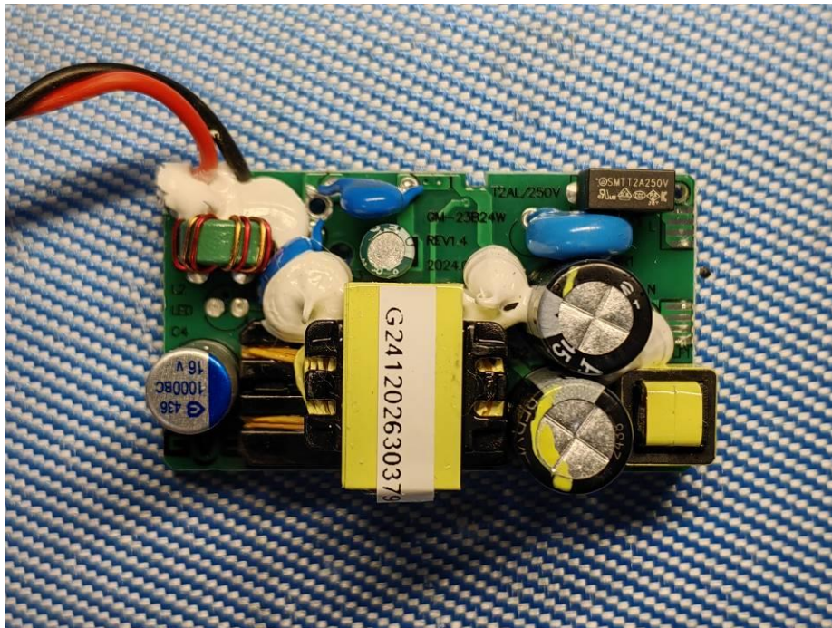
Picture 17_ Adapter GMB24-120200-1A
