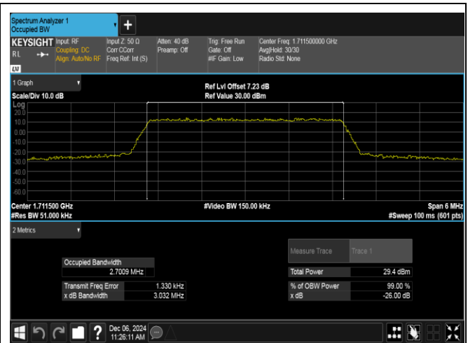
Band66-3MHz-16QAM-131987-15RB#0-PASS
