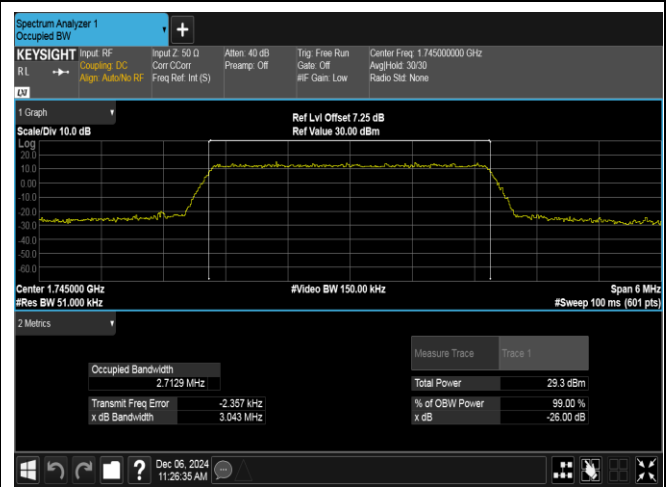
Band66-3MHz-16QAM-132322-15RB#0-PASS
