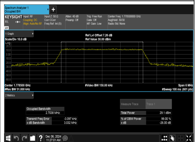
Band66-3MHz-16QAM-132657-15RB#0-PASS
