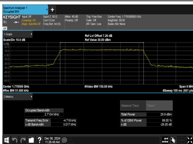
Band66-3MHz-QPSK-132657-15RB#0-PASS
