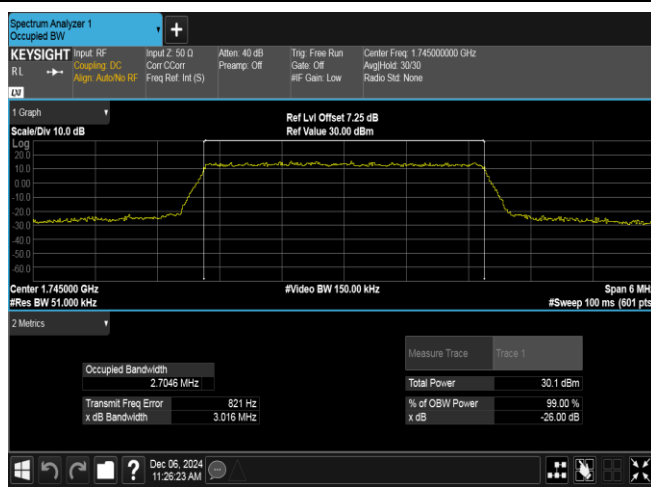
Band66-3MHz-QPSK-132322-15RB#0-PASS
