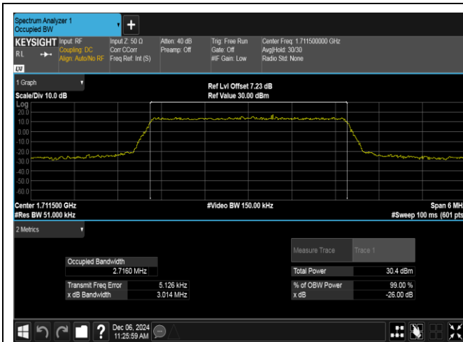
Band66-3MHz-QPSK-131987-15RB#0-PASS
