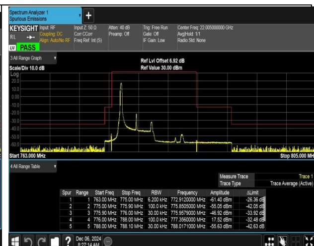
Band13_5MHz_16QAM_23205_1RB#0
