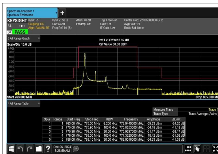
Band13_5MHz_QPSK_23205_1RB#0
