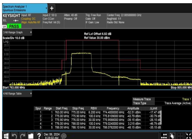
Band13_5MHz_QPSK_23205_25RB#0
