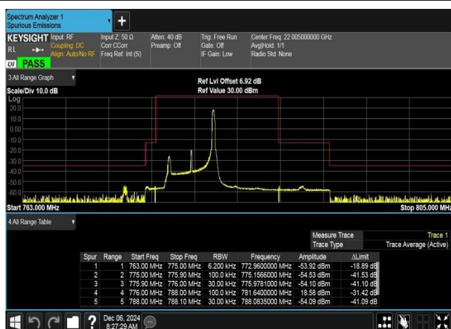
Band13_5MHz_QPSK_23205_1RB#24
