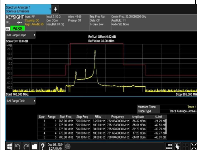
Band13_5MHz_16QAM_23205_1RB#24
