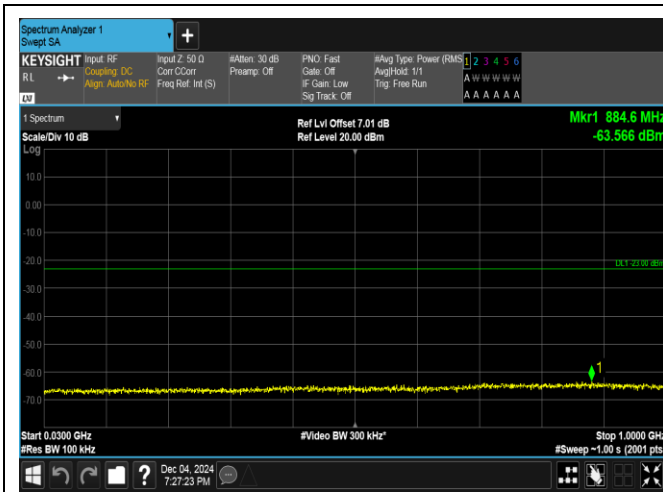
Band4_10MHz_16QAM_20000_50RB#0_30~1000_30~1000
