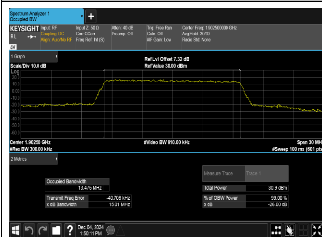
Band2-15MHz-QPSK-19125-75RB#0-PASS
