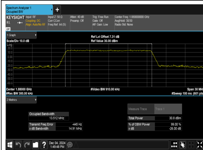
Band2-15MHz-QPSK-18900-75RB#0-PASS
