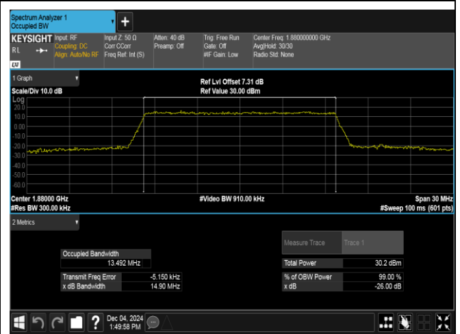
Band2-15MHz-16QAM-18900-75RB#0-PASS
