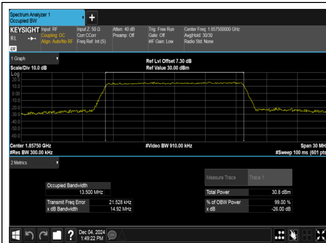
Band2-15MHz-QPSK-18675-75RB#0-PASS
