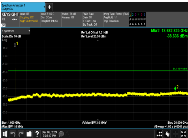
Band4-1413-2-1000~20000MHz-PASS
