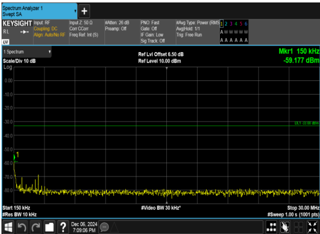
Band4-1413-4-0.15~30MHz-PASS
