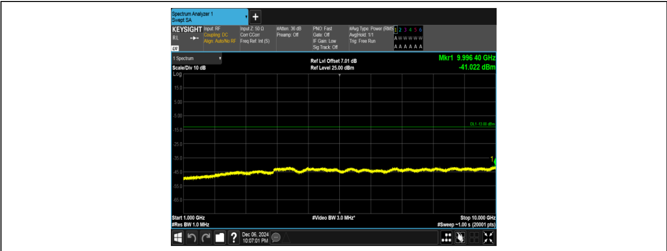
Band5-4132-4-1000~10000MHz-PASS
