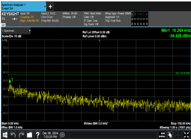
Band4-1513-1-0.009~0.15MHz-PASS
