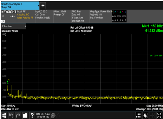
Band5-4132-2-0.15~30MHz-PASS
