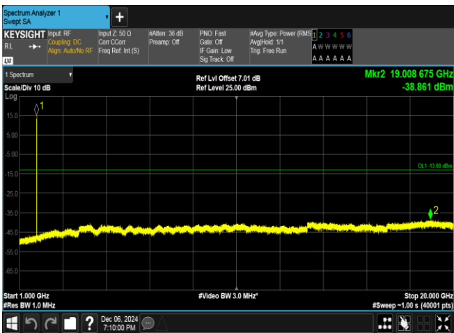
Band4-1513-4-1000~20000MHz-PASS
