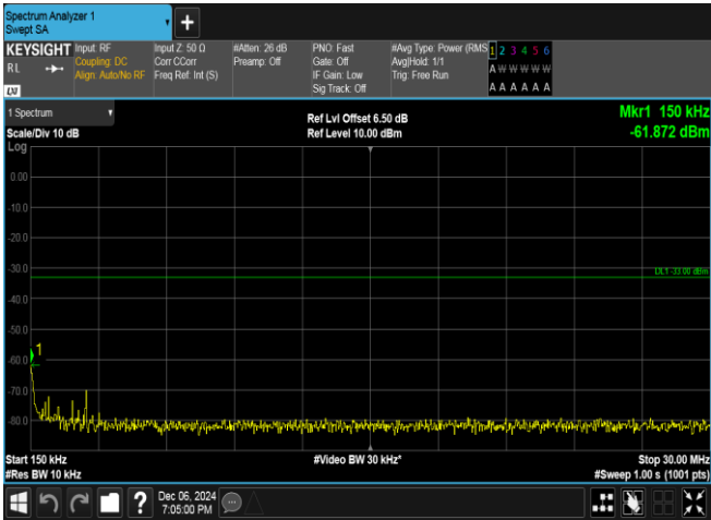
Band4-1413-2-0.15~30MHz-PASS
