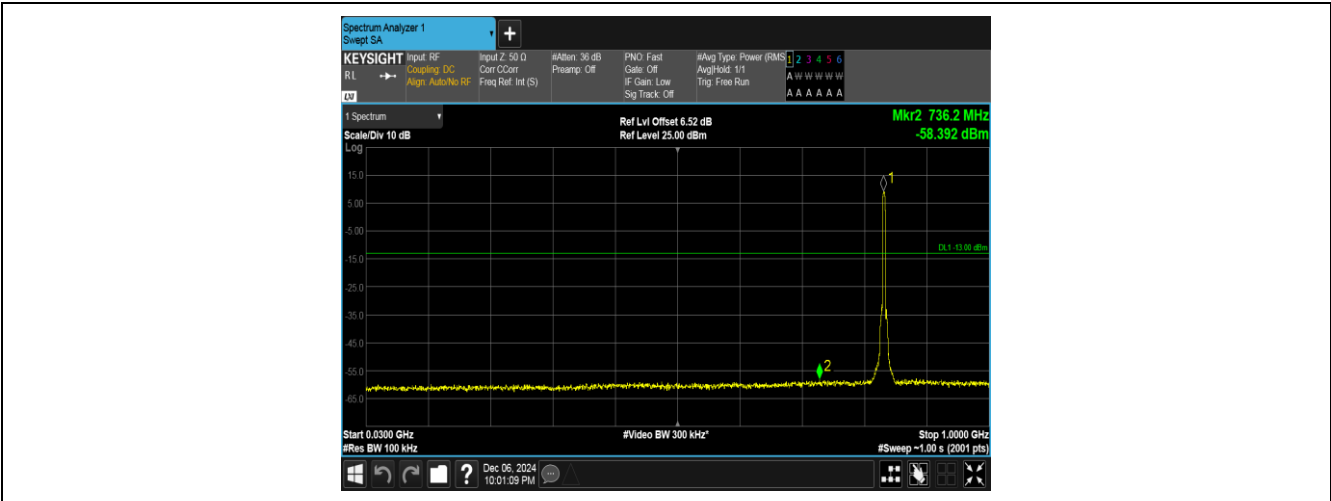
Band5-4182-1-30~1000MHz-PASS
