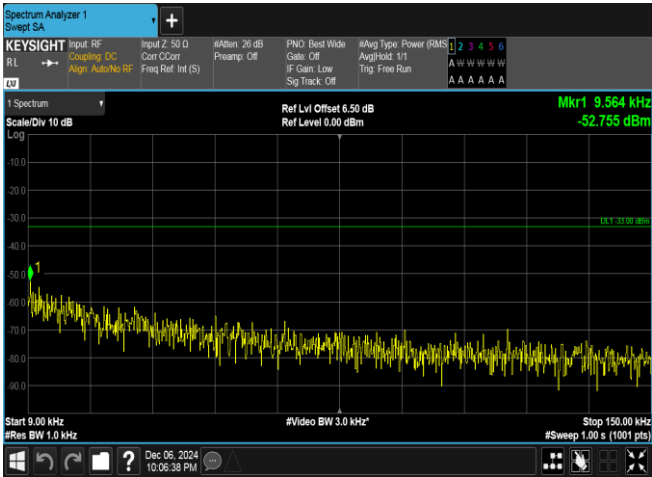
Band5-4132-4-0.009~0.15MHz-PASS
