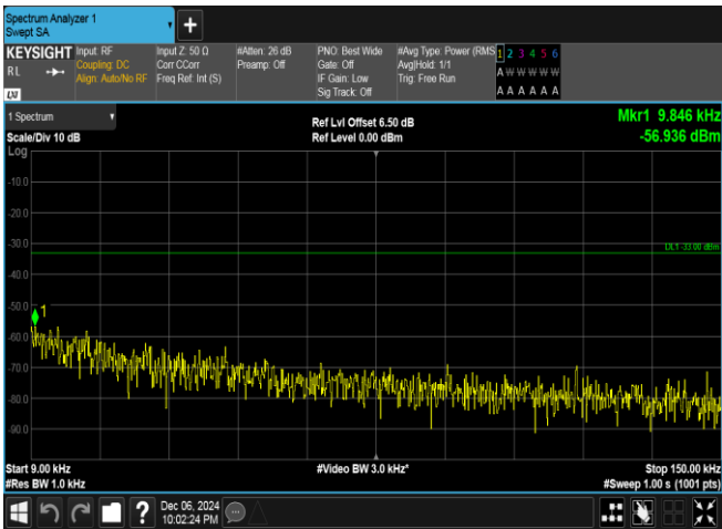
Band5-4132-2-0.009~0.15MHz-PASS
