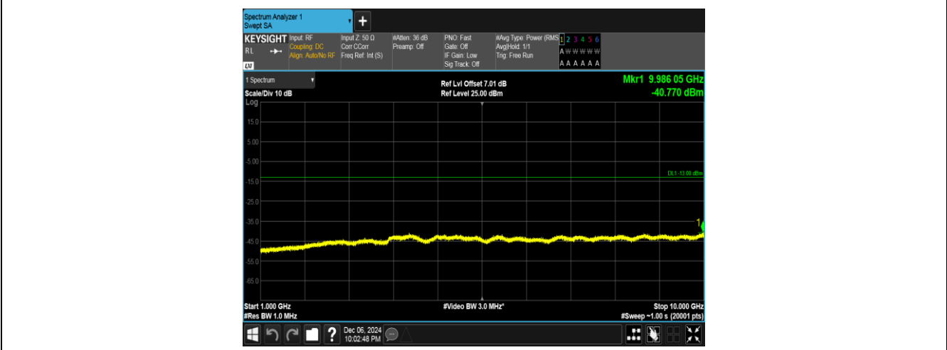
Band5-4132-2-1000~10000MHz-PASS
