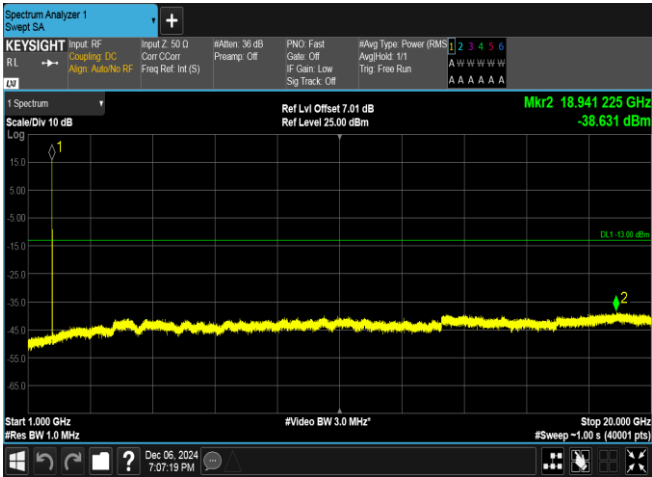
Band4-1413-3-1000~20000MHz-PASS
