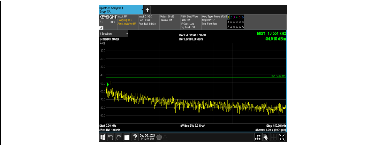
Band4-1513-2-0.009~0.15MHz-PASS
