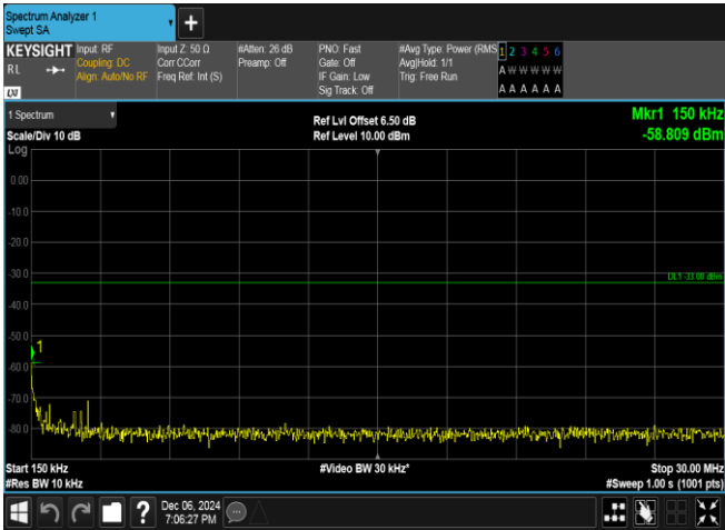
Band4-1312-3-0.15~30MHz-PASS
