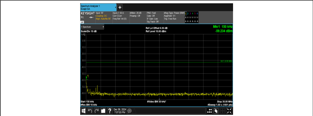
Band4-1413-3-0.15~30MHz-PASS
