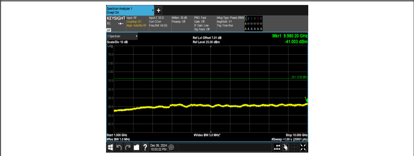
Band5-4182-2-1000~10000MHz-PASS
