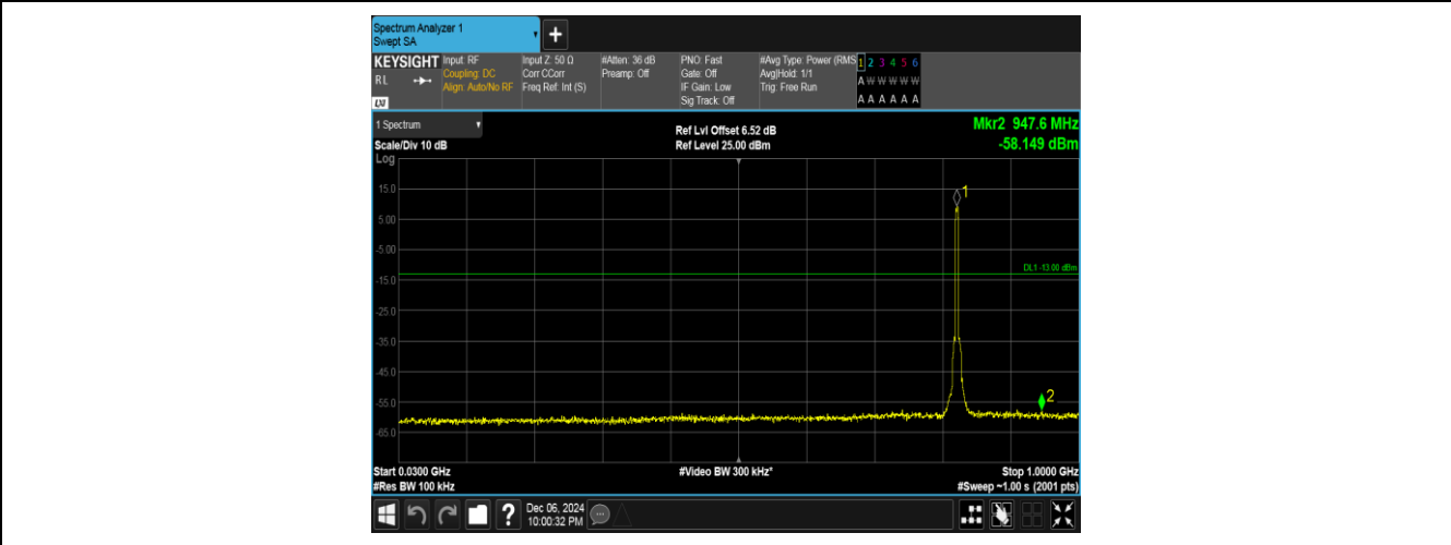
Band5-4132-1-30~1000MHz-PASS
