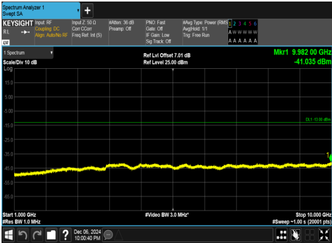
Band5-4132-1-1000~10000MHz-PASS
