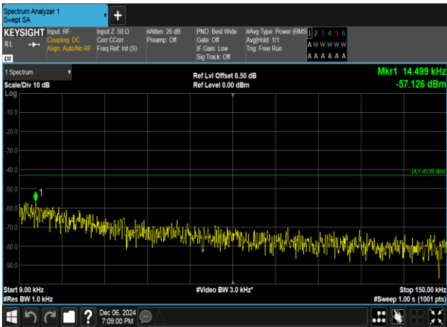
Band4-1413-4-0.009~0.15MHz-PASS
