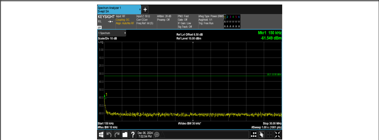
Band4-1413-1-0.15~30MHz-PASS
