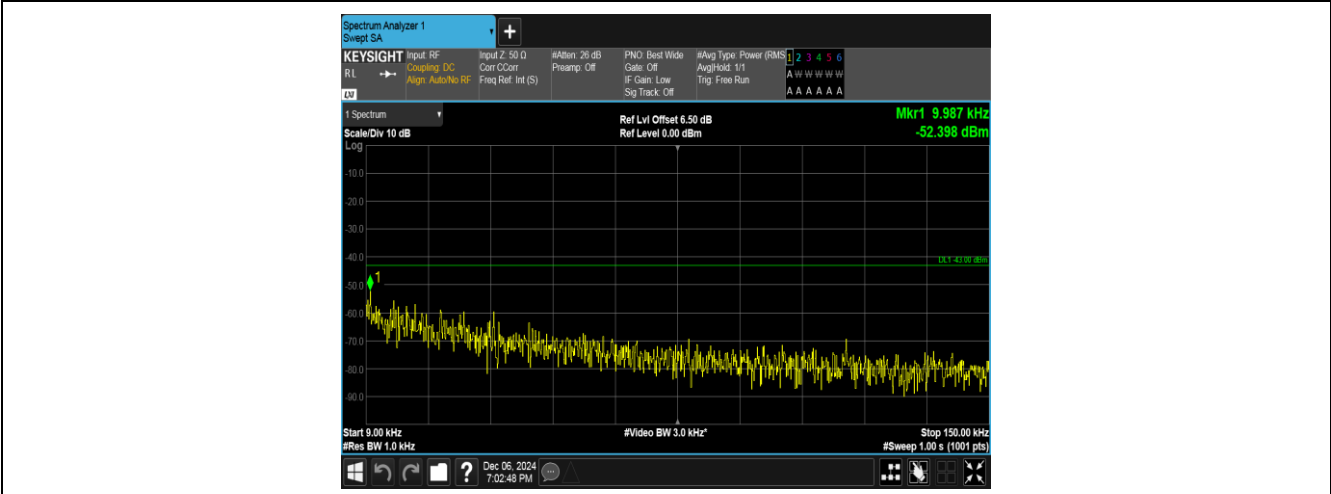
Band4-1413-1-0.009~0.15MHz-PASS
