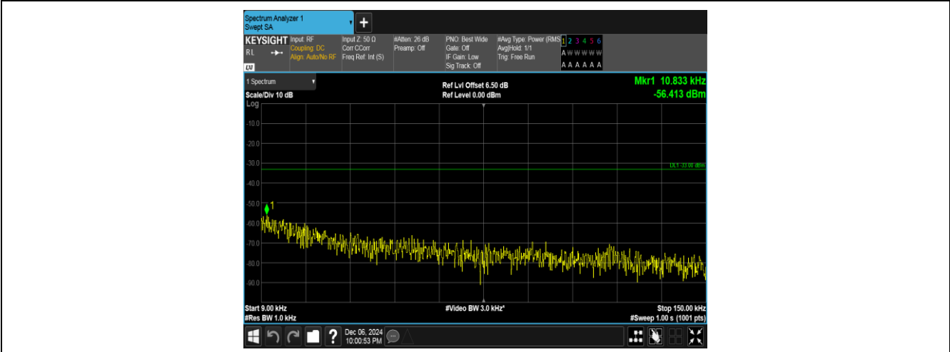
Band5-4182-1-0.009~0.15MHz-PASS
