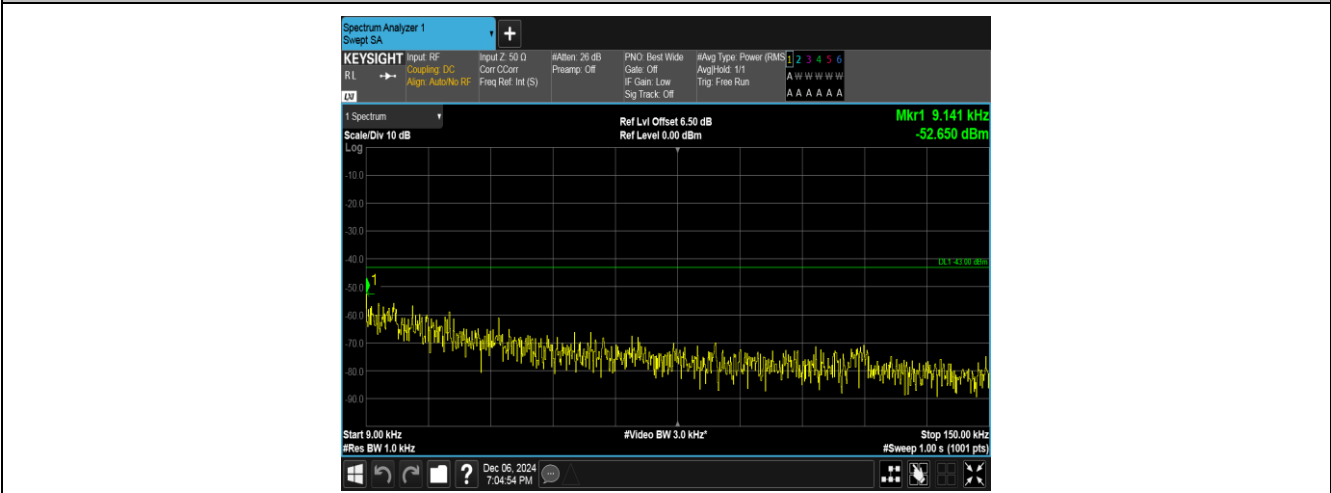
Band4-1413-2-0.009~0.15MHz-PASS
