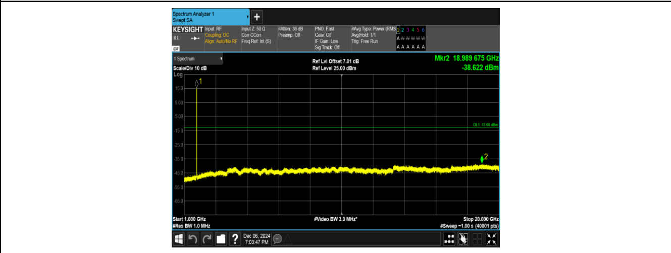
Band4-1513-1-1000~20000MHz-PASS
