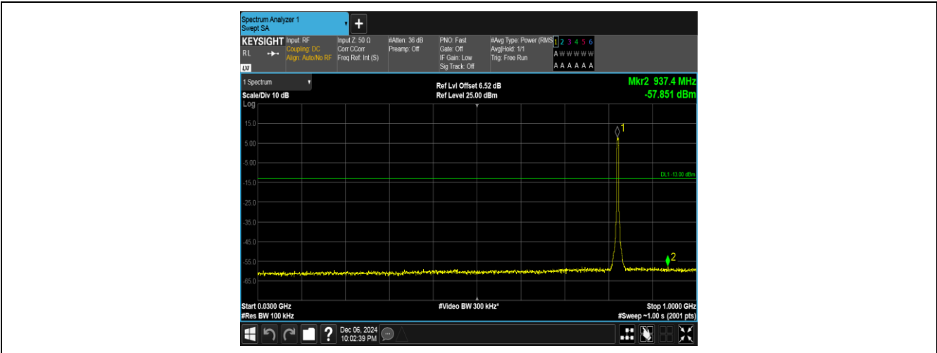
Band5-4132-2-30~1000MHz-PASS
