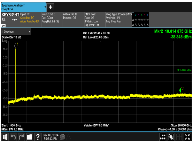
Band4-1312-3-1000~20000MHz-PASS
