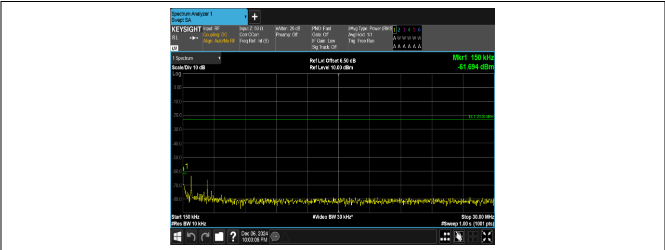
Band5-4182-2-0.15~30MHz-PASS
