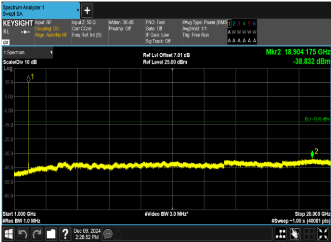
Band2-9262-1-1000~20000MHz-PASS
