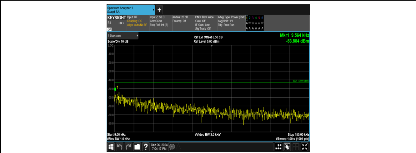
Band4-1312-2-0.009~0.15MHz-PASS
