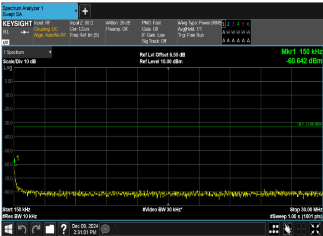
Band2-9262-2-0.15~30MHz-PASS
