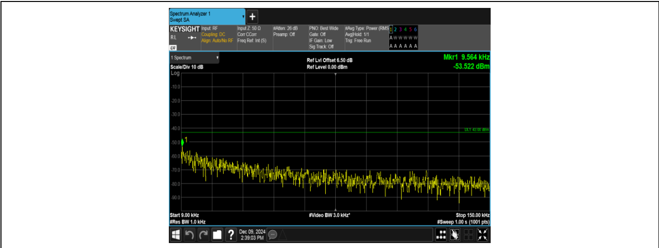
Band2-9400-5-0.009~0.15MHz-PASS
