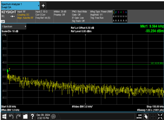
Band2-9538-2-0.009~0.15MHz-PASS
