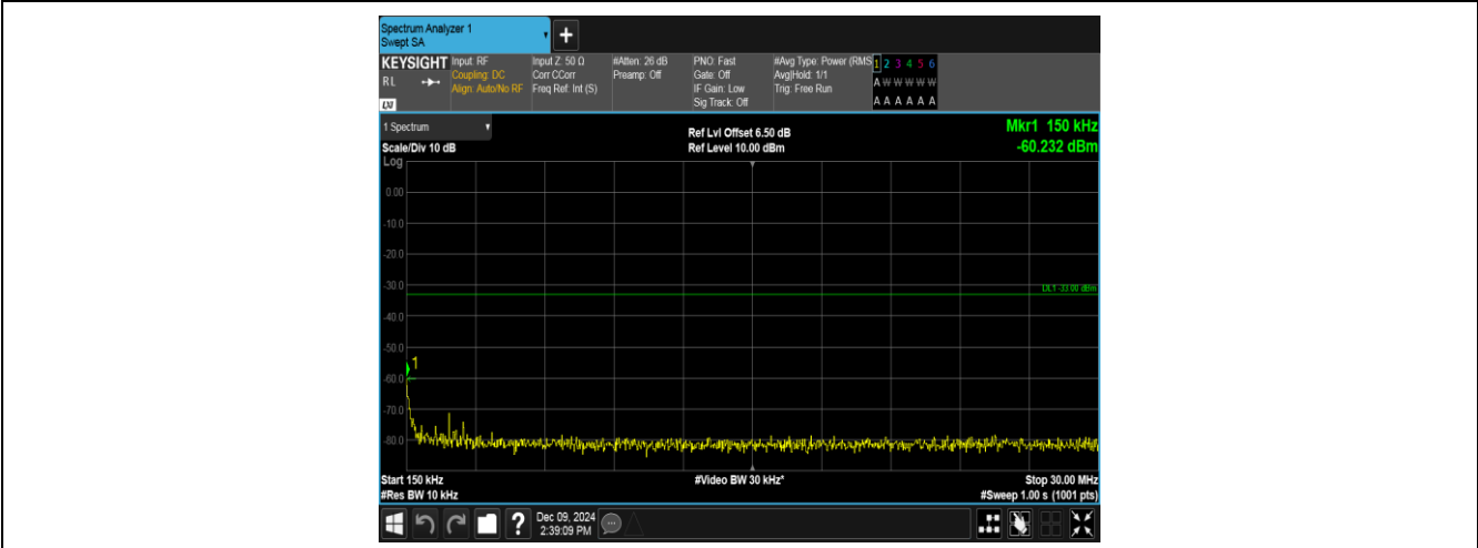
Band2-9400-5-0.15~30MHz-PASS
