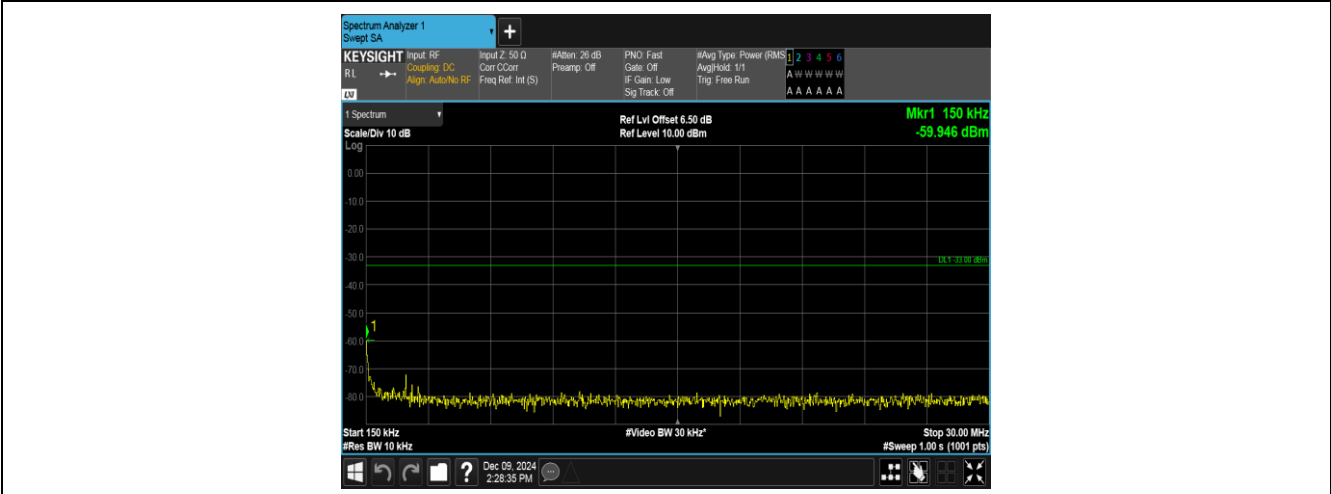
Band2-9262-1-0.15~30MHz-PASS
