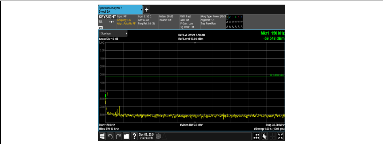
Band2-9400-4-0.15~30MHz-PASS
