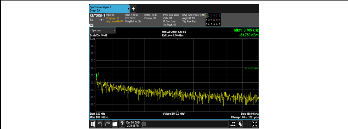
Band2-9538-5-0.009~0.15MHz-PASS
