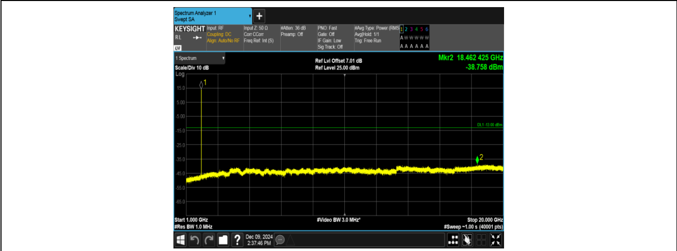
Band2-9538-4-1000~20000MHz-PASS
