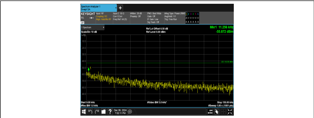
Band4-1312-1-0.009~0.15MHz-PASS
