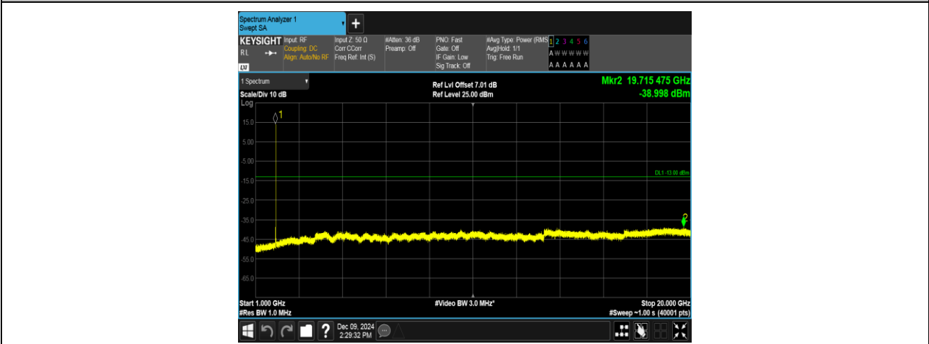
Band2-9400-1-1000~20000MHz-PASS
