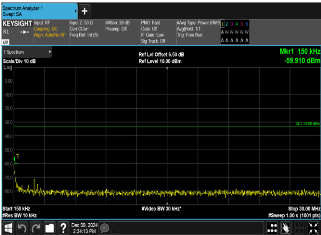
Band2-9400-3-0.15~30MHz-PASS
