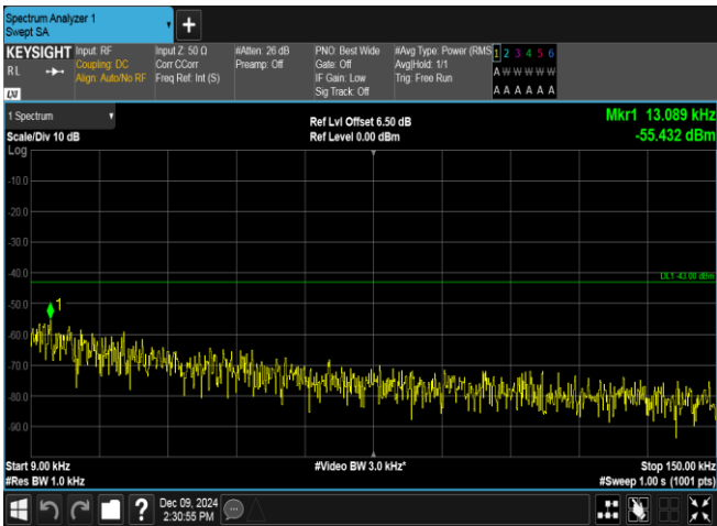
Band2-9262-2-0.009~0.15MHz-PASS
