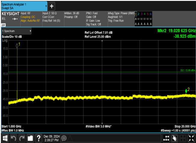
Band2-9400-5-1000~20000MHz-PASS
