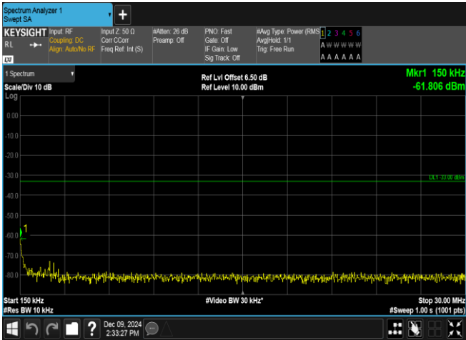
Band2-9262-3-0.15~30MHz-PASS
