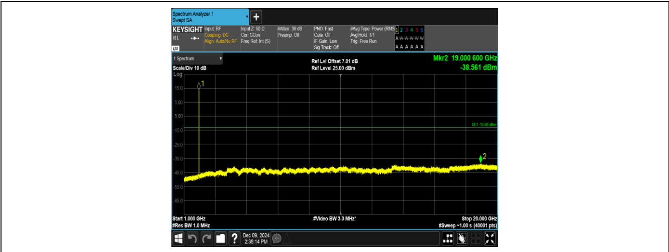
Band2-9538-3-1000~20000MHz-PASS
