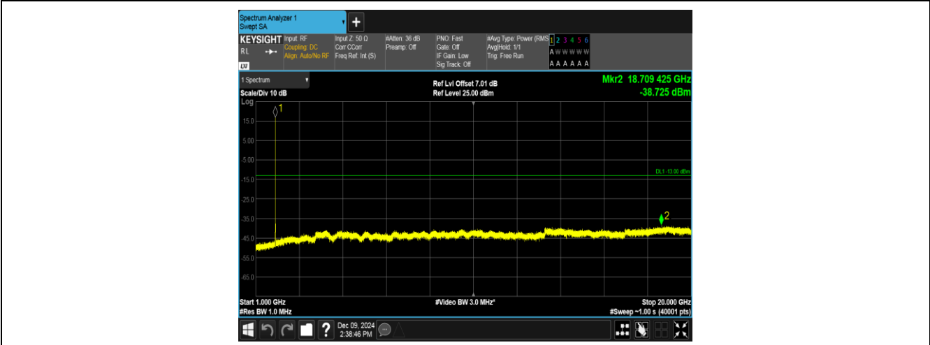
Band2-9262-5-1000~20000MHz-PASS
