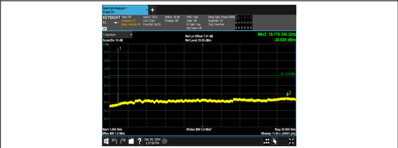
Band2-9400-4-1000~20000MHz-PASS
