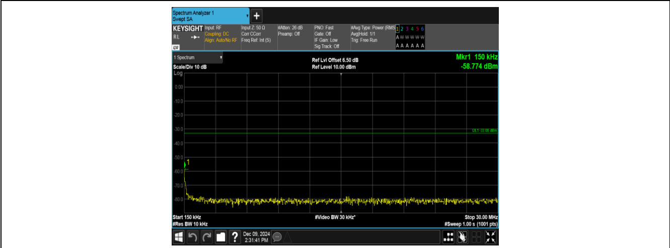
Band2-9400-2-0.15~30MHz-PASS
