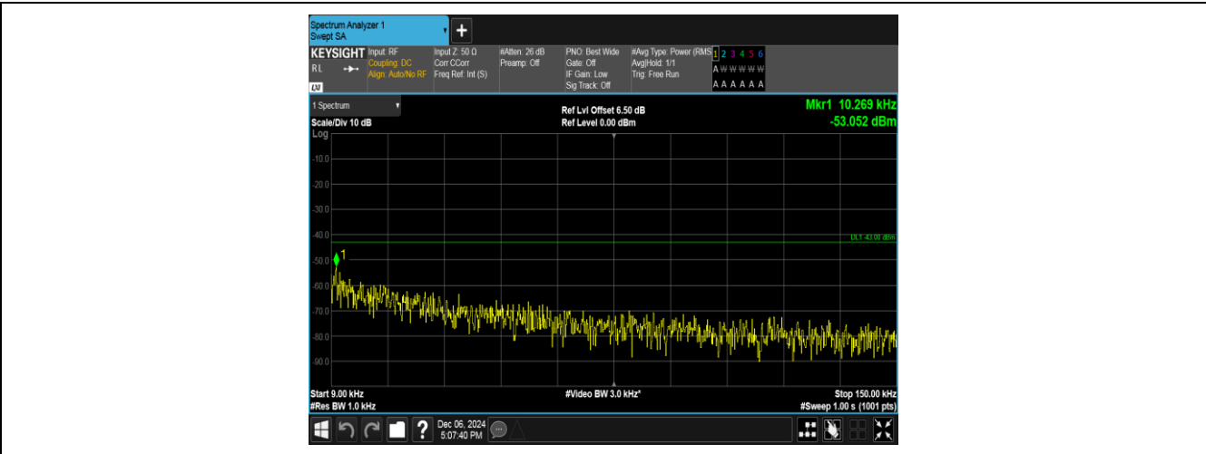
Band2-9538-2-0.009~0.15MHz-PASS
