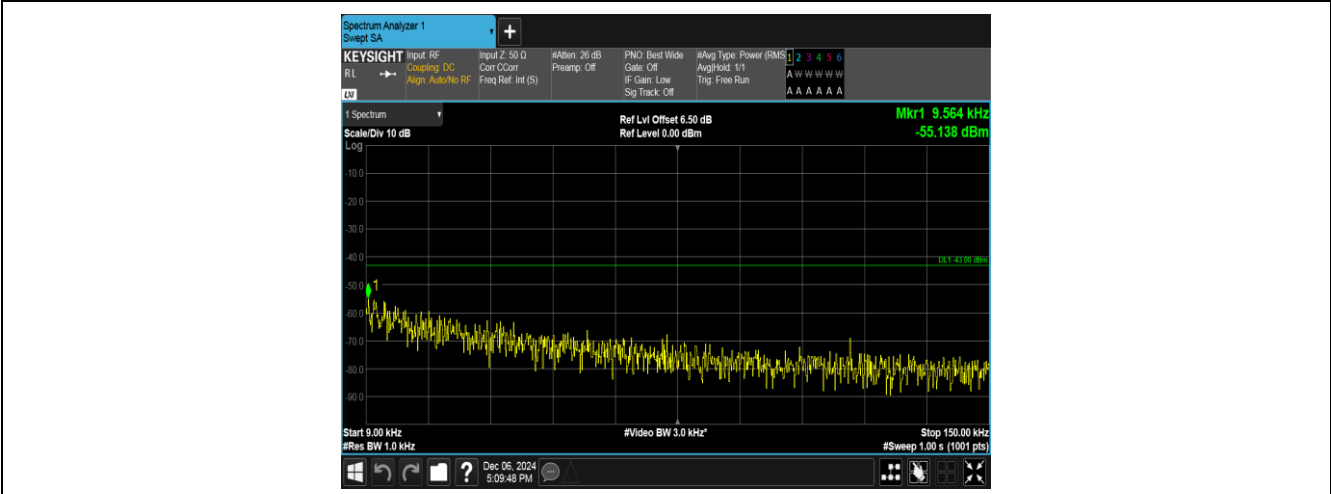
Band2-9538-3-0.009~0.15MHz-PASS
