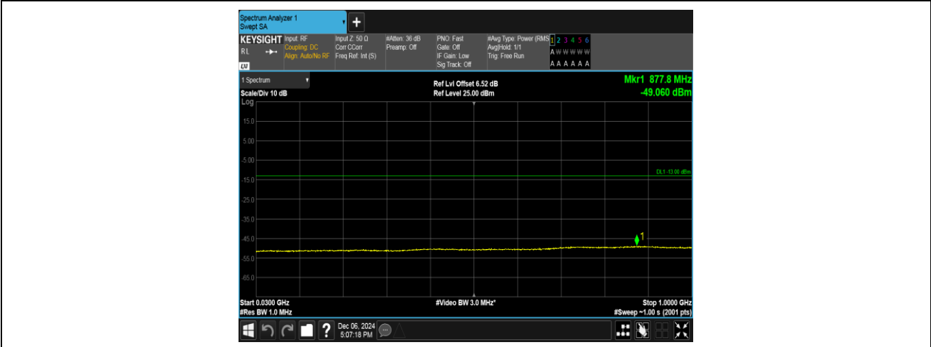
Band2-9400-2-30~1000MHz-PASS
