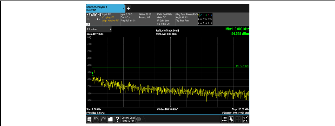
Band2-9400-3-0.009~0.15MHz-PASS
