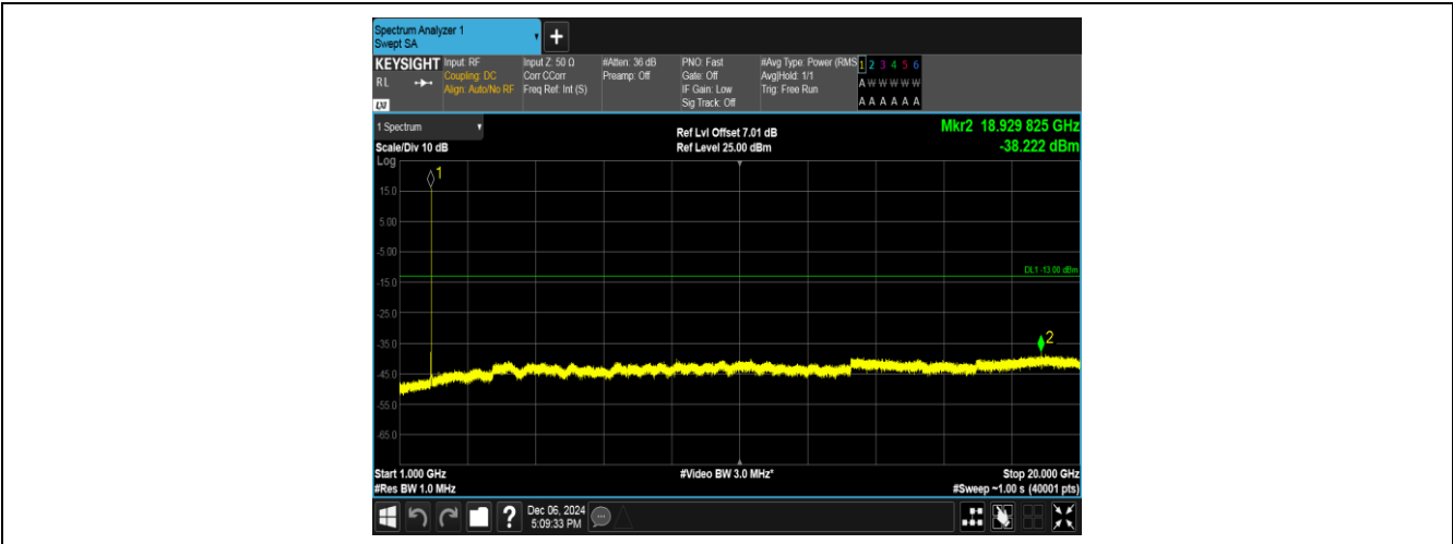
Band2-9400-3-1000~20000MHz-PASS
