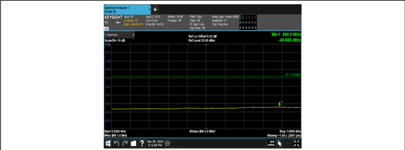
Band2-9538-4-30~1000MHz-PASS
