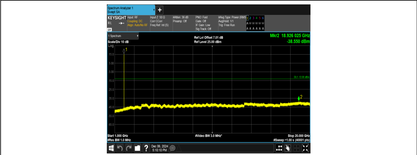
Band2-9538-3-1000~20000MHz-PASS
