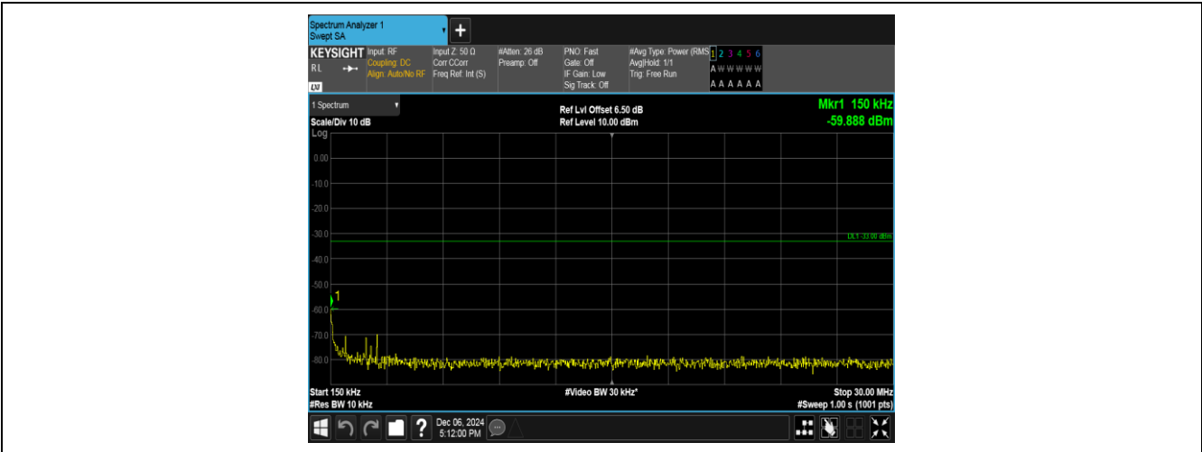
Band2-9538-4-0.15~30MHz-PASS
