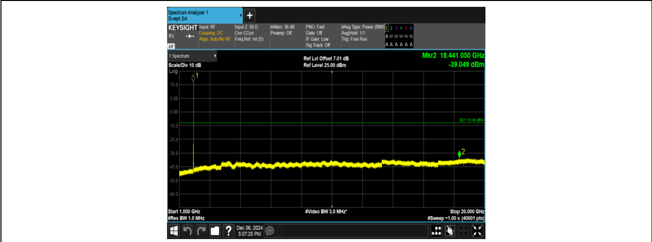
Band2-9400-2-1000~20000MHz-PASS
