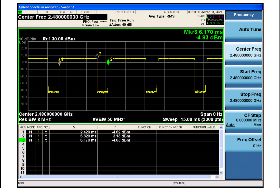
EDR-π /4-DQPSK-ANT1-2480
