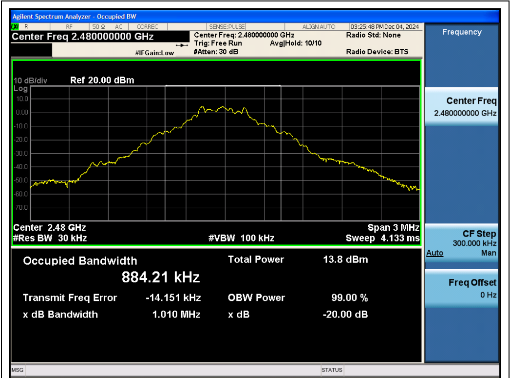
Test_Graph_BR_ANT1_2480_1Mbps_OBW
