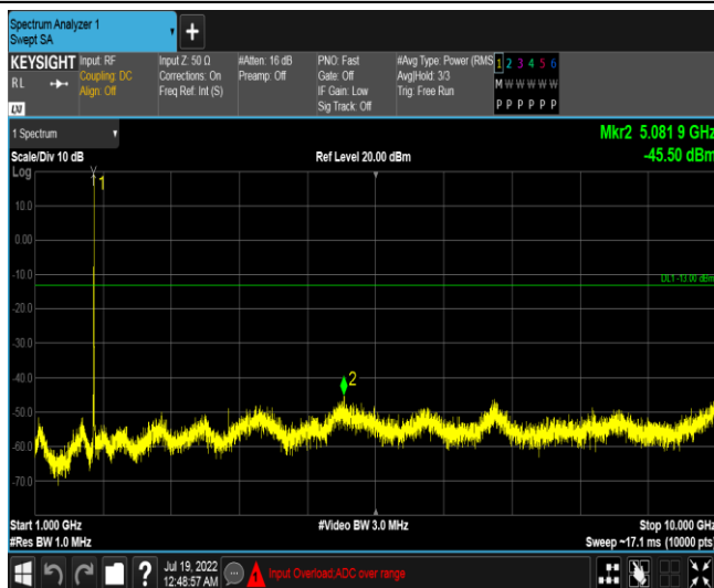
Band66-5MHz-16QAM-132647-1RB#0-Range5:1000~10000MHz
