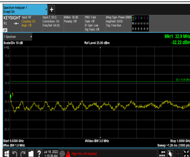
Band66-10MHz-QPSK-132022-1RB#0-Range1:30~1000MHz
