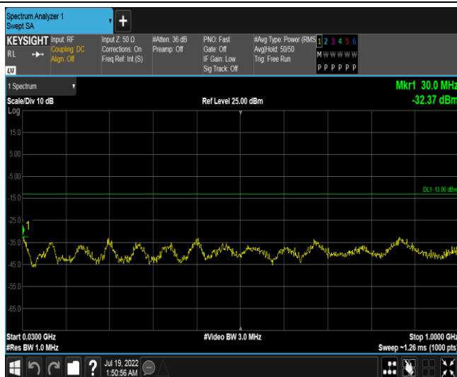
Band66-15MHz-QPSK-132597-1RB#0-Range4:30~1000MHz
