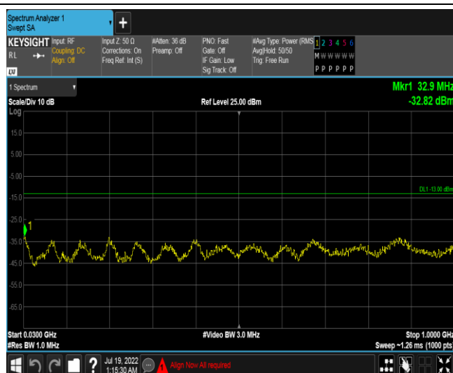
Band66-10MHz-QPSK-132622-1RB#0-Range1:30~1000MHz
