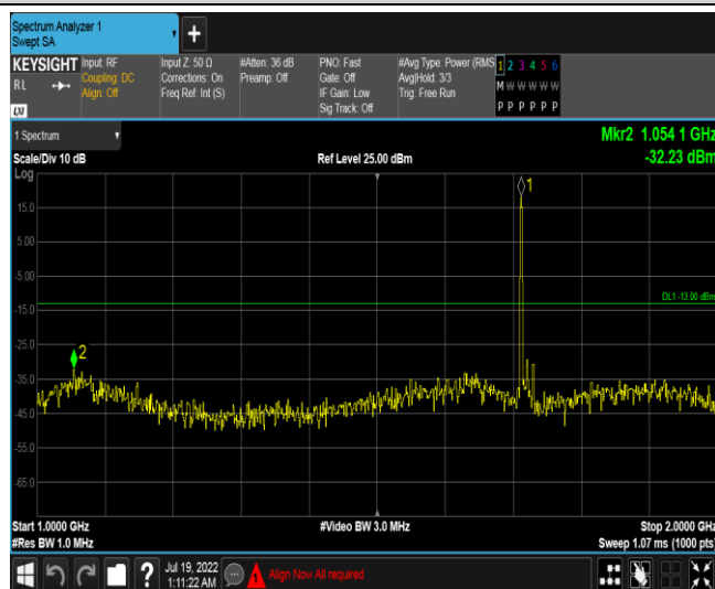
Band66-10MHz-16QAM-132022-1RB#0-Range2:1000~2000MHz
