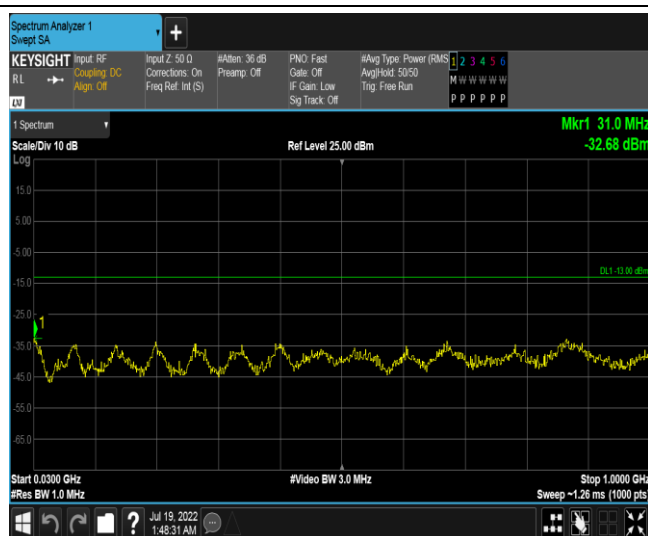
Band66-15MHz-QPSK-132322-1RB#0-Range4:30~1000MHz
