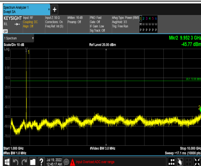
Band66-5MHz-QPSK-132322-1RB#0-Range5:1000~10000MHz
