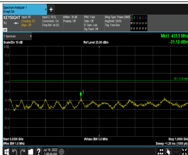
Band66-15MHz-16QAM-132322-1RB#0-Range4:30~1000MHz
