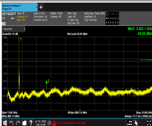
Band66-15MHz-16QAM-132047-1RB#0-Range5:1000~10000MHz
