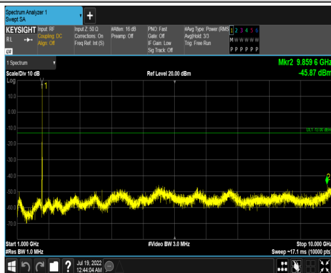
Band66-5MHz-16QAM-131997-1RB#0-Range5:1000~10000MHz
