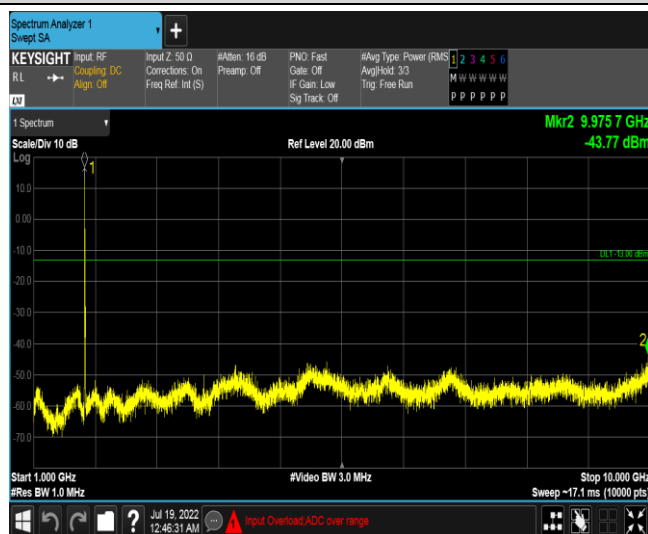
Band66-5MHz-16QAM-132322-1RB#0-Range5:1000~10000MHz
