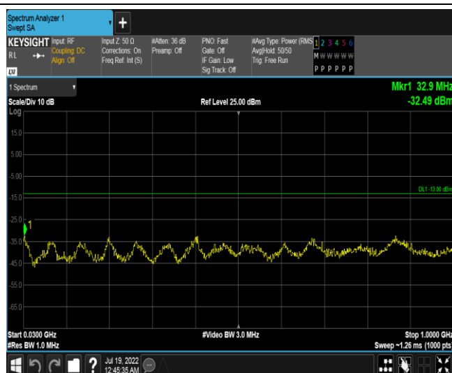
Band66-5MHz-16QAM-132322-1RB#0-Range4:30~1000MHz
