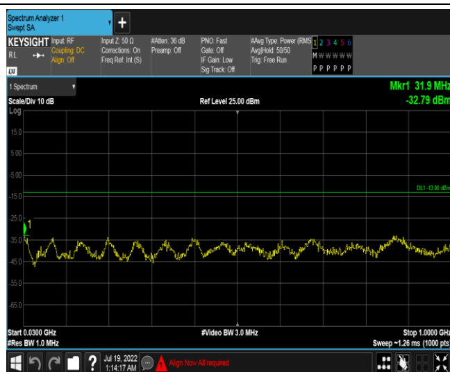
Band66-10MHz-16QAM-132322-1RB#0-Range1:30~1000MHz
