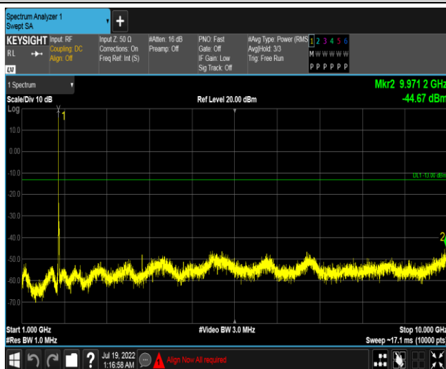
Band66-10MHz-16QAM-132622-1RB#0-Range5:1000~10000MHz
