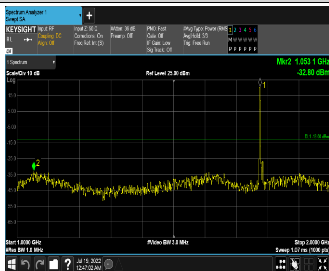
Band66-5MHz-QPSK-132647-1RB#0-Range2:1000~2000MHz
