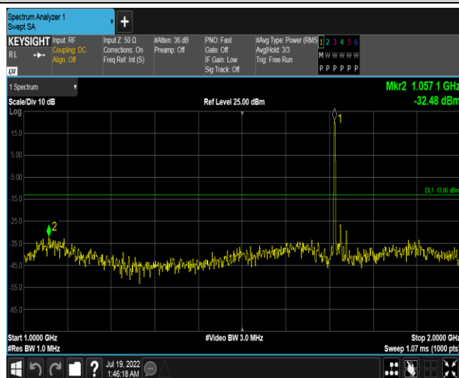
Band66-15MHz-QPSK-132047-1RB#0-Range2:1000~2000MHz
