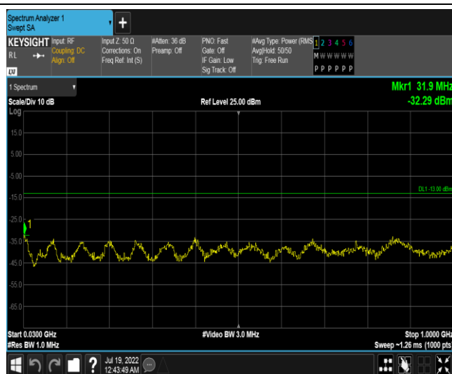
Band66-5MHz-16QAM-131997-1RB#0-Range1:30~1000MHz
