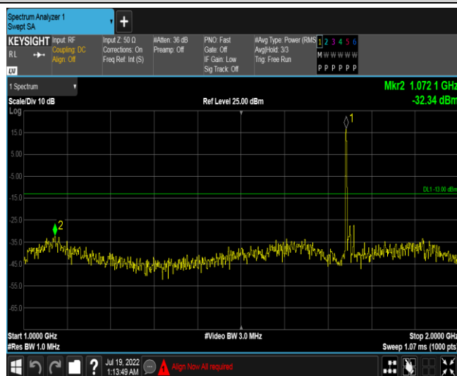
Band66-10MHz-16QAM-132322-1RB#0-Range2:1000~2000MHz
