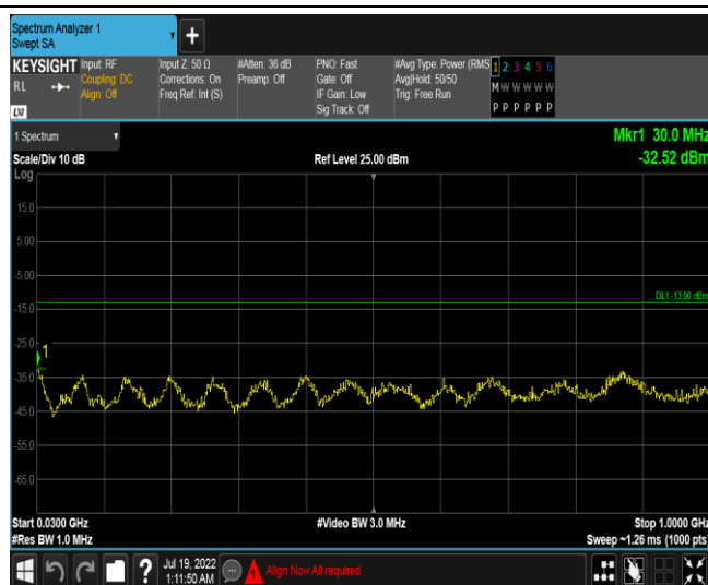
Band66-10MHz-16QAM-132022-1RB#0-Range1:30~1000MHz
