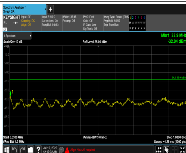
Band66-3MHz-QPSK-132657-1RB#0-Range4:30~1000MHz
