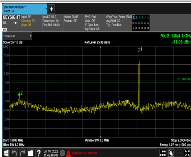
Band66-1.4MHz-16QAM-131979-1RB#0-Range2:1000~2000MHz
