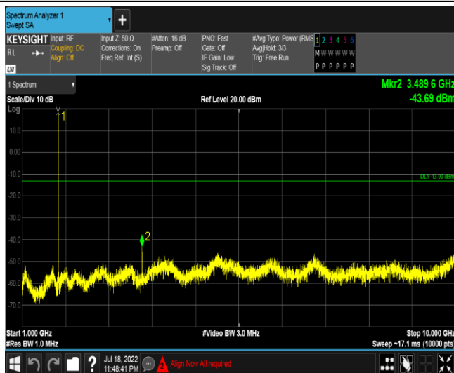
Band66-1.4MHz-QPSK-132322-1RB#0-Range5:1000~10000MHz
