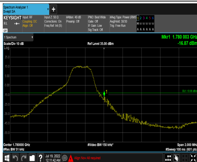
Band66-3MHz-16QAM-132657-1RB#14
