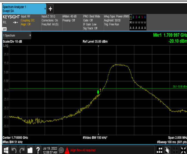
Band66-3MHz-QPSK-131987-1RB#0
