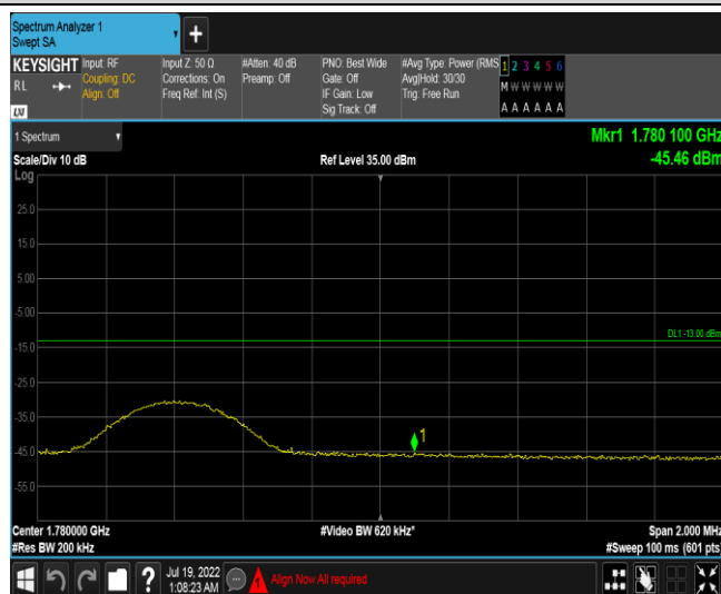
Band66-10MHz-16QAM-132622-1RB#0
