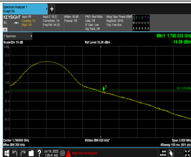
Band66-10MHz-QPSK-132622-1RB#49
