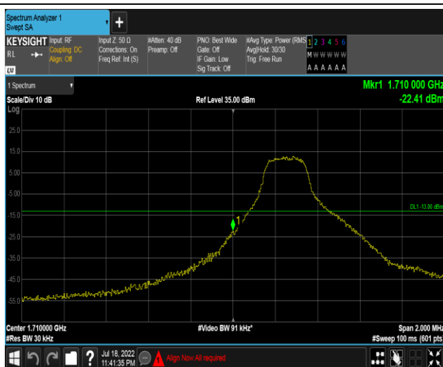
Band66-1.4MHz-QPSK-131979-1RB#5
