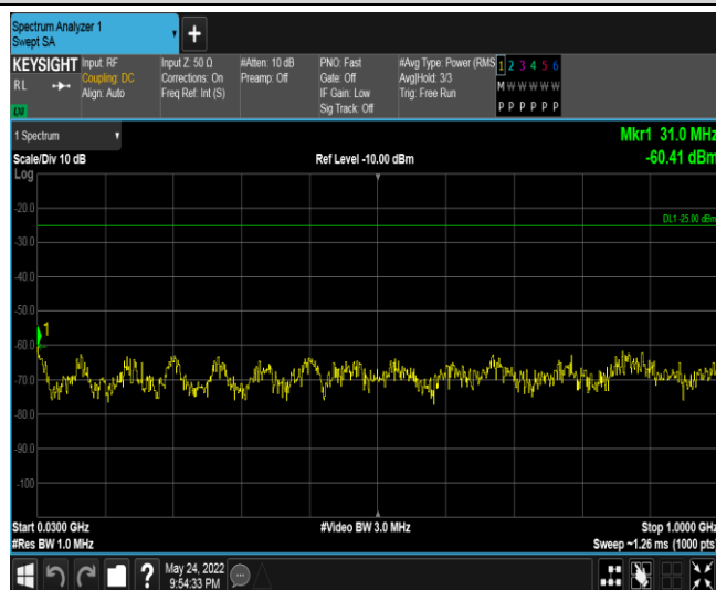
Band41-5MHz-16QAM-39675-1RB#0-Range1:30~1000MHz
