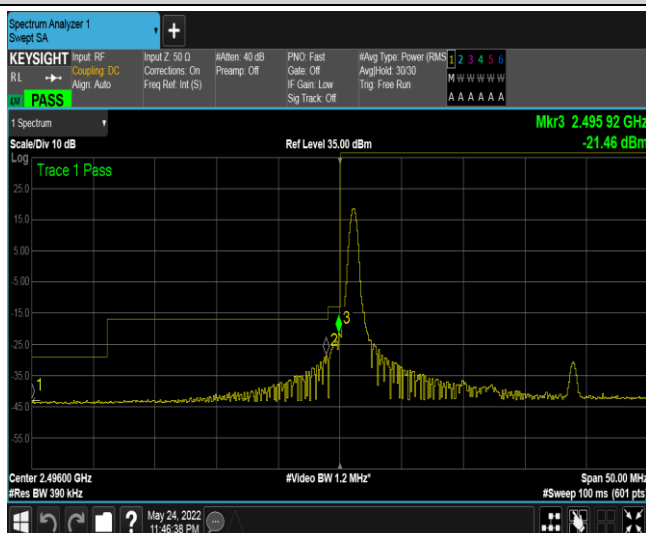
Band41-20MHz-16QAM-39750-1RB#99
