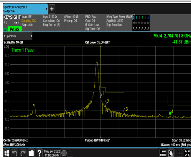
Band41-15MHz-QPSK-41515-1RB#74
