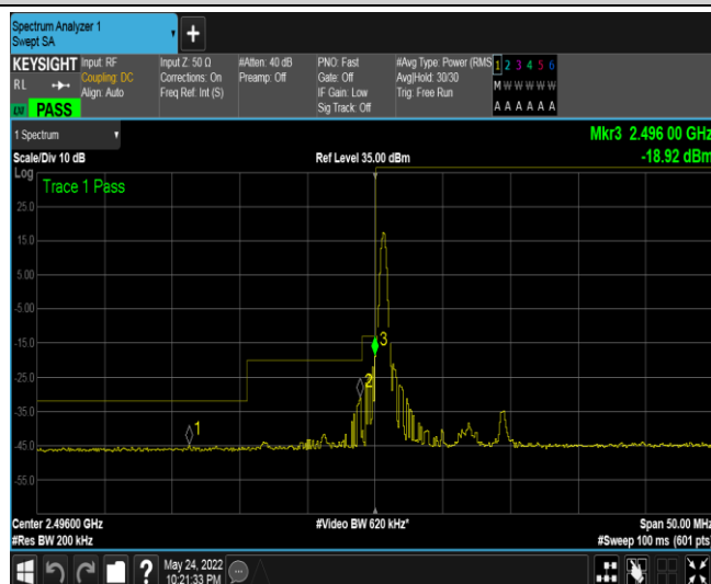
Band41-10MHz-QPSK-39700-1RB#49
