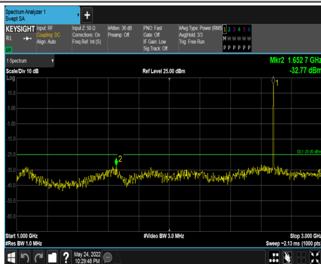
Band41-10MHz-16QAM-41540-1RB#0-Range2:1000~3000MHz
