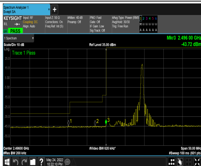
Band41-10MHz-QPSK-39700-1RB#49
