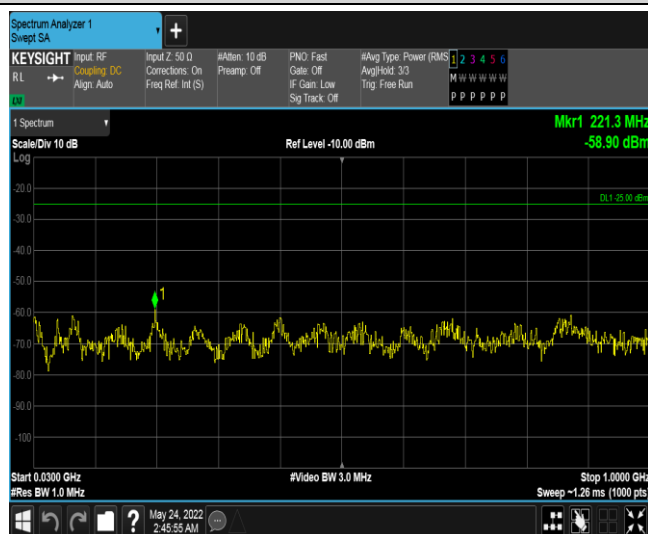
Band38-15MHz-QPSK-38000-1RB#0-Range1:30~1000MHz
