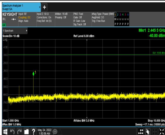
Band26-15MHz-QPSK-26765-1RB#0-Range3:1000~10000MHz
