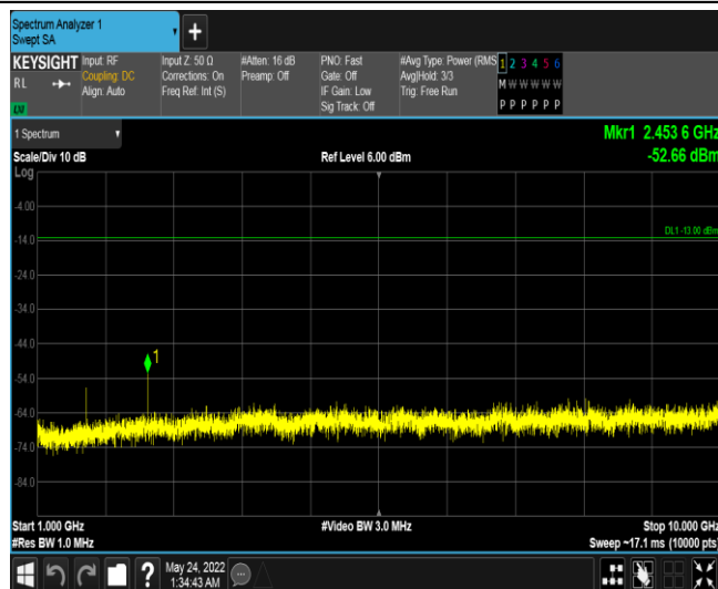
Band26-3MHz-16QAM-26740-1RB#0-Range3:1000~10000MHz
