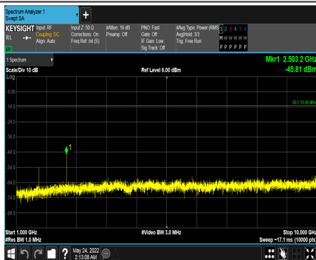
Band26-5MHz-16QAM-26915-1RB#0-Range3:1000~10000MHz
