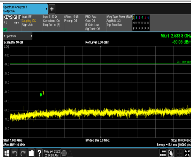
Band26-5MHz-QPSK-27015-1RB#0-Range3:1000~10000MHz
