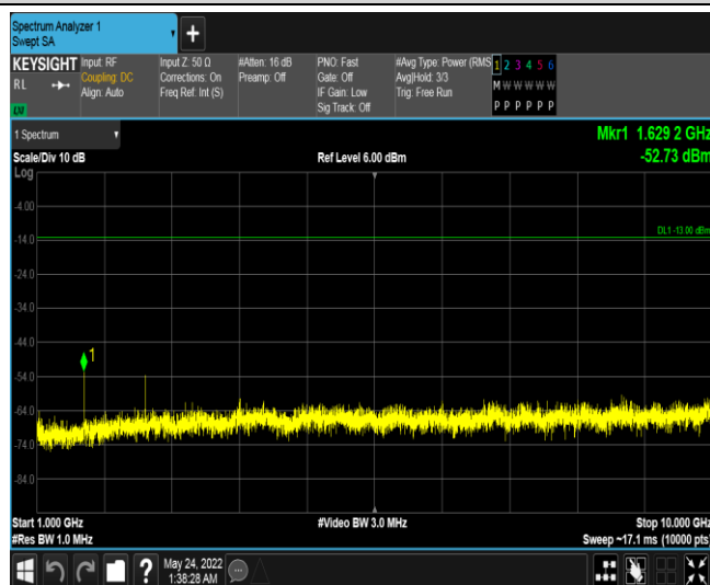
Band26-5MHz-QPSK-26715-1RB#0-Range3:1000~10000MHz
