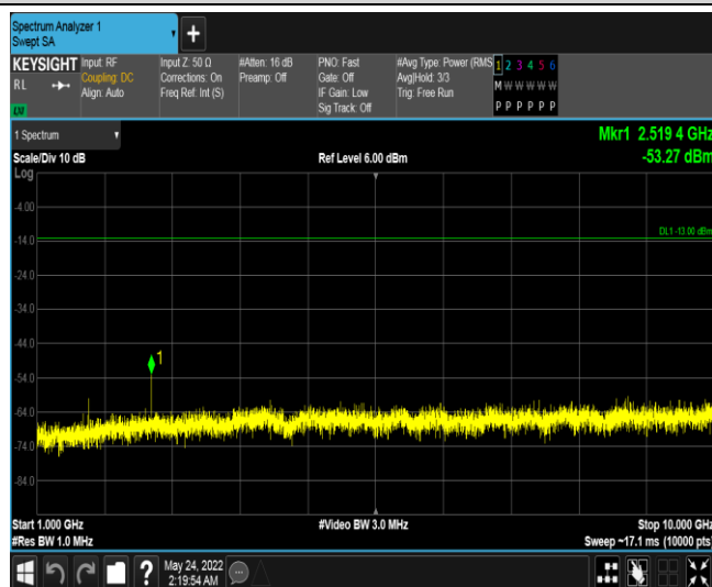
Band26-10MHz-QPSK-26990-1RB#0-Range3:1000~10000MHz
