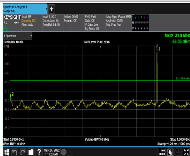
Band26-1.4MHz-QPSK-26740-1RB#0-Range2:30~1000MHz
