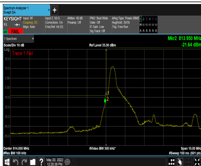
Band26-5MHz-16QAM-26715-1RB#24
