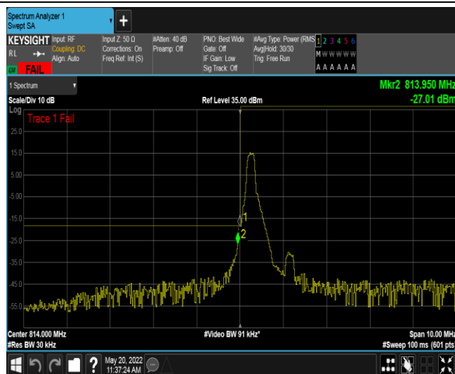
Band26-1.4MHz-QPSK-26697-1RB#5
