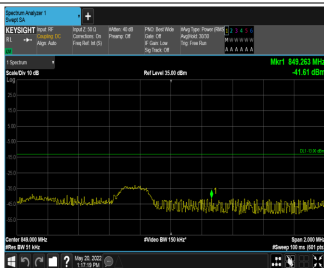
Band26-3MHz-16QAM-27025-1RB#14
