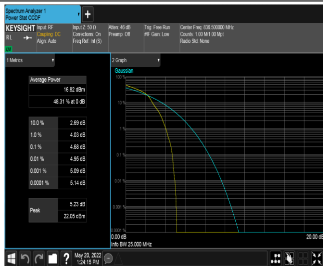
Band26-3MHz-16QAM-26915-1RB#0
