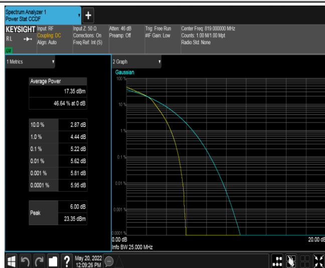
Band26-3MHz-16QAM-26740-15RB#0
