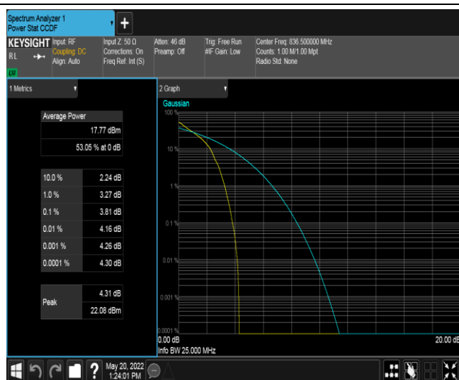
Band26-3MHz-QPSK-26915-15RB#0
