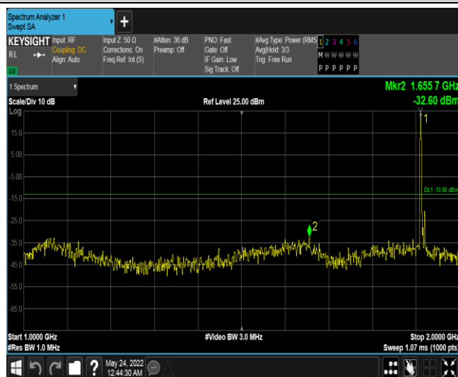
Band25-5MHz-16QAM-26665-1RB#0-Range2:1000~2000MHz
