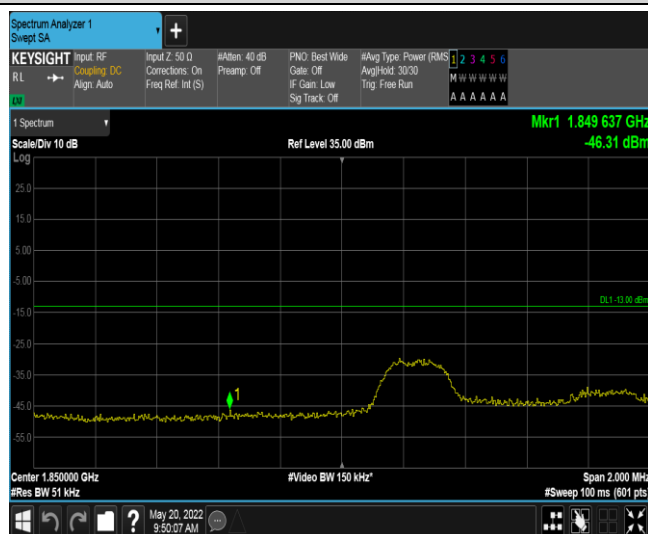
Band25-3MHz-16QAM-26055-1RB#14
