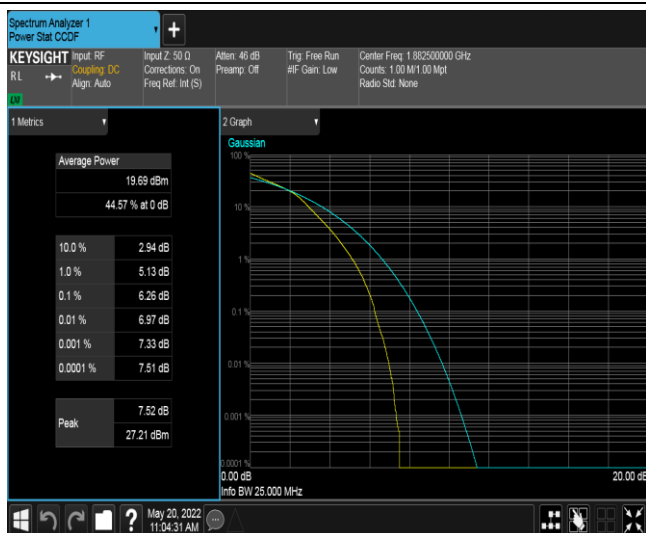
Band25-15MHz-16QAM-26615-1RB#0
