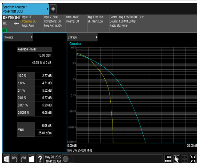
Band25-10MHz-16QAM-26090-50RB#0
