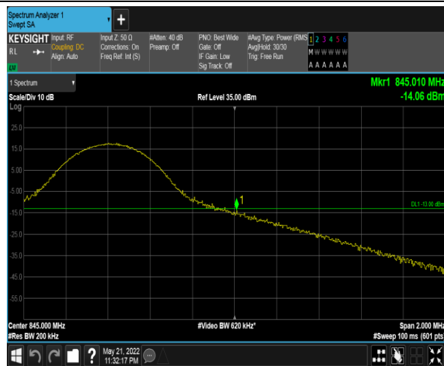
Band19-10MHz-16QAM-24100-1RB#49
