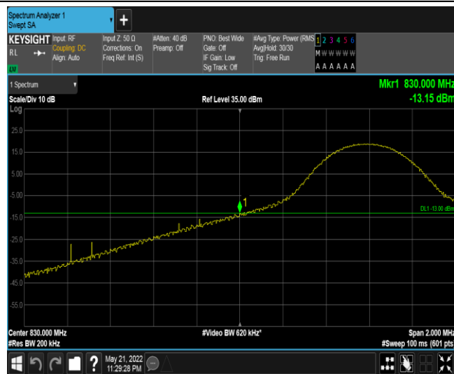
Band19-10MHz-QPSK-24050-1RB#0
