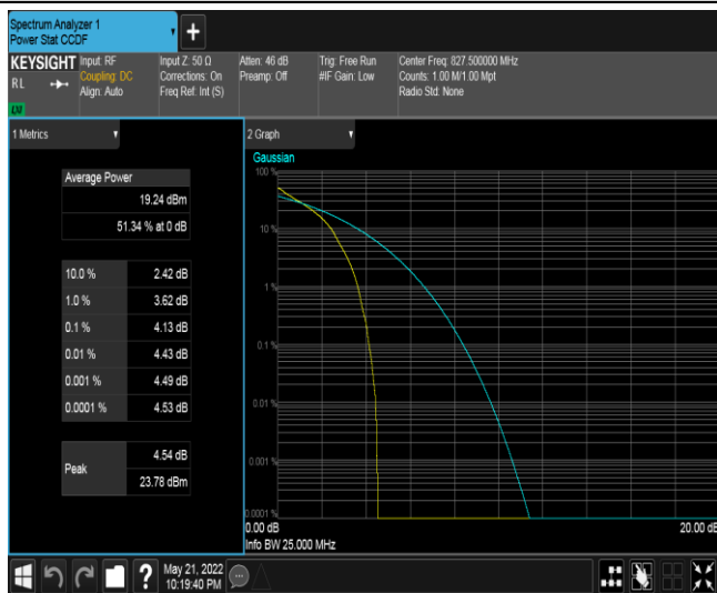
Band18-5MHz-QPSK-23975-1RB#0
