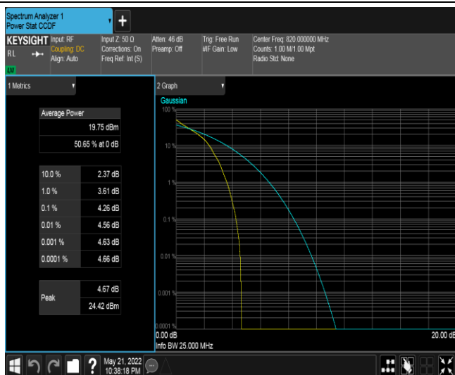
Band18-10MHz-QPSK-23900-50RB#0
