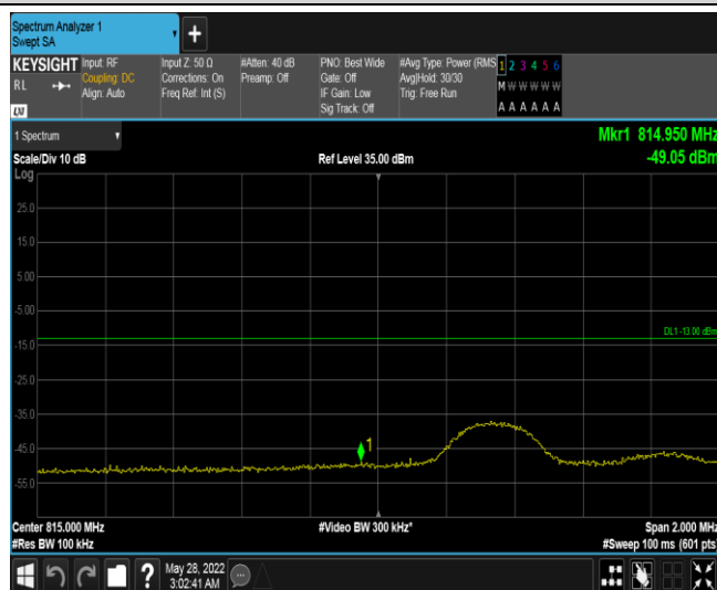
Band18-5MHz-16QAM-23875-1RB#24
