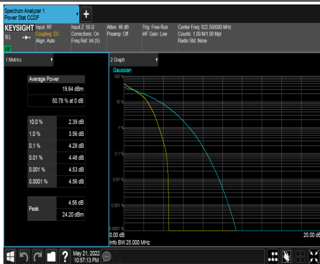
Band18-15MHz-QPSK-23925-1RB#0
