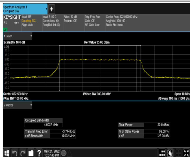
Band18-5MHz-16QAM-23925-25RB#0
