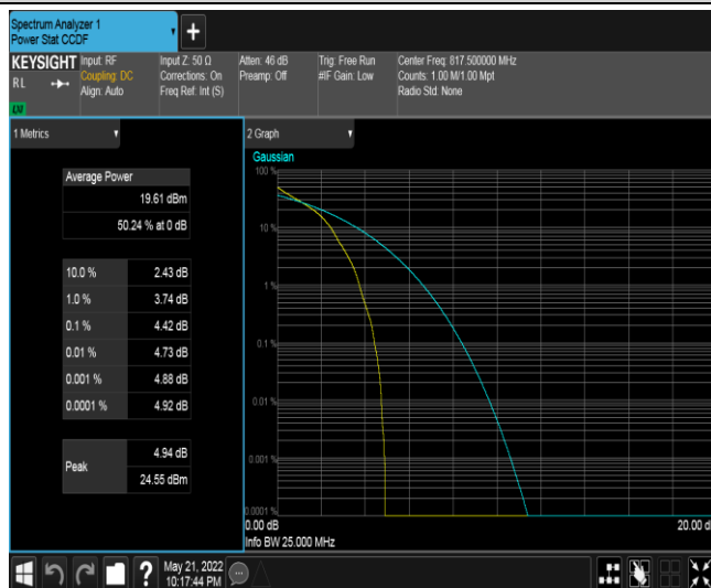
Band18-5MHz-QPSK-23875-25RB#0
