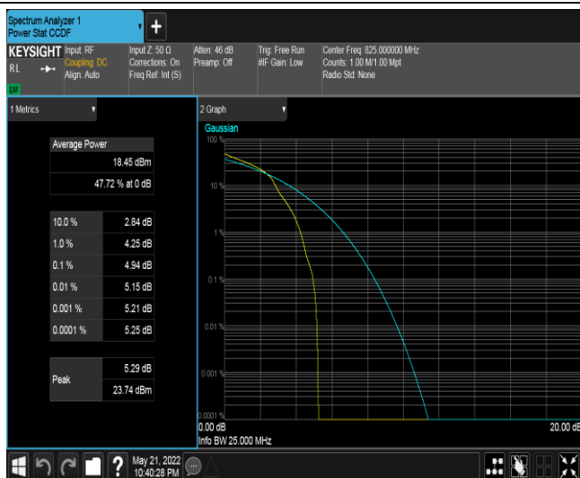
Band18-10MHz-16QAM-23950-50RB#0
