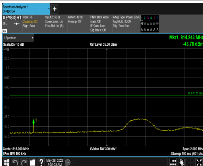
Band18-5MHz-QPSK-23875-25RB#0
