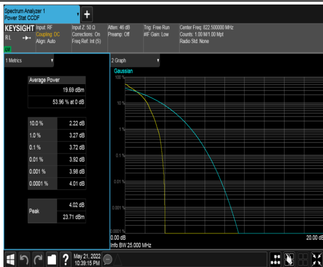
Band18-10MHz-QPSK-23925-1RB#0
