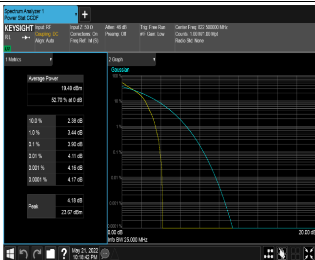
Band18-5MHz-QPSK-23925-25RB#0
