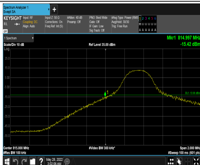
Band18-5MHz-16QAM-23875-1RB#24
