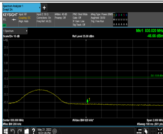
Band18-10MHz-16QAM-23950-1RB#49
