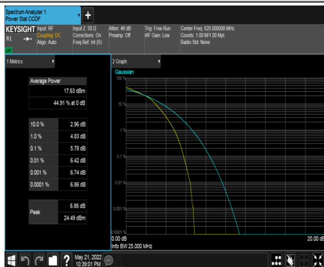
Band18-10MHz-16QAM-23900-50RB#0
