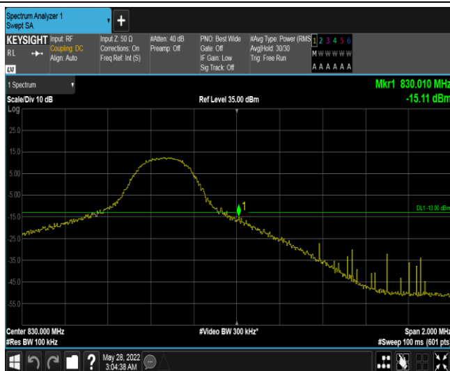
Band18-5MHz-16QAM-23975-25RB#0
