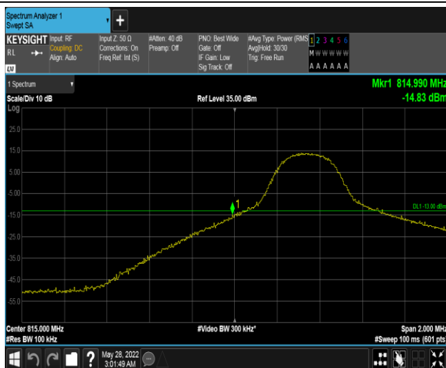
Band18-5MHz-QPSK-23875-1RB#24
