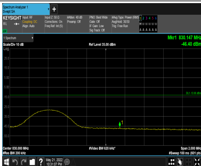
Band18-10MHz-QPSK-23950-1RB#49
