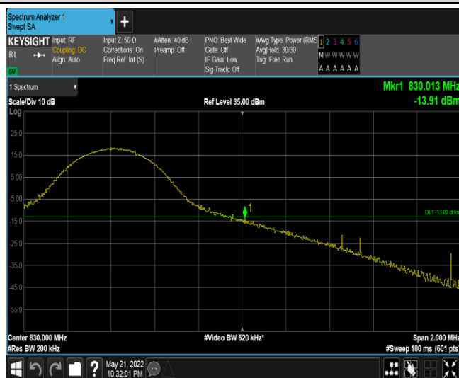
Band18-10MHz-16QAM-23950-1RB#49
