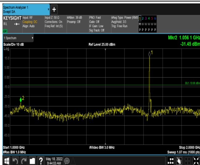
Band4-5MHz-16QAM-20175-1RB#0-Range2:1000~2000MHz
