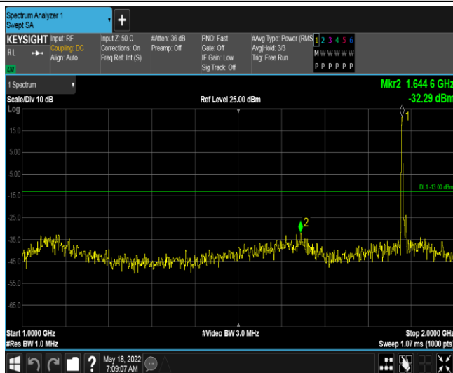
Band2-5MHz-16QAM-18900-1RB#0-Range2:1000~2000MHz
