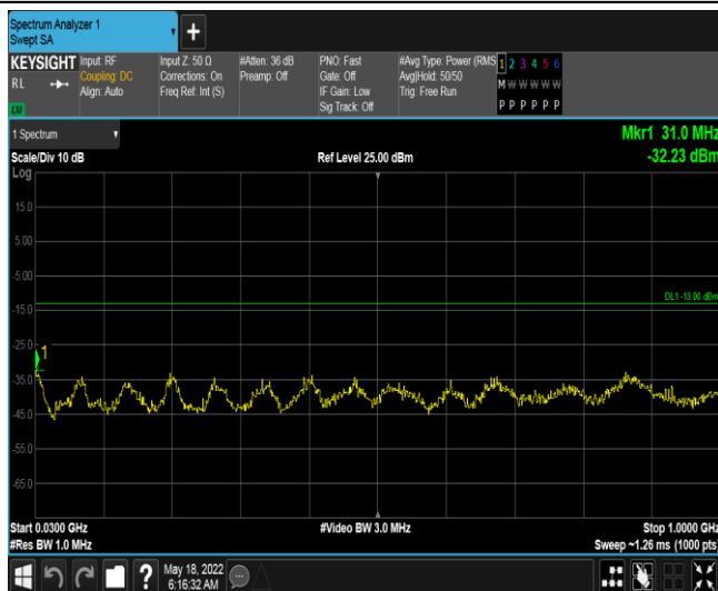
Band2-1.4MHz-16QAM-18607-1RB#0-Range1:30~1000MHz
