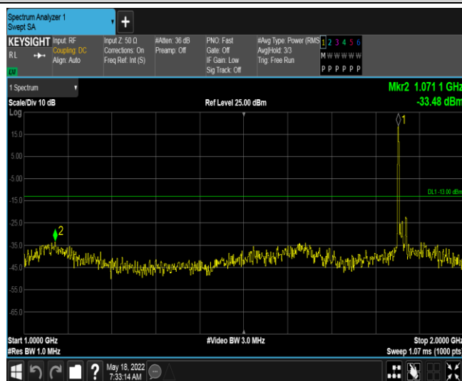
Band2-10MHz-16QAM-18650-1RB#0-Range2:1000~2000MHz
