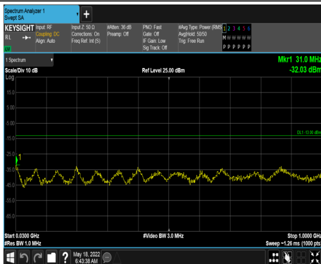
Band2-3MHz-QPSK-19185-1RB#0-Range1:30~1000MHz
