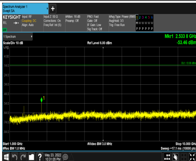
Band5-5MHz-QPSK-20625-1RB#0-Range3:1000~10000MHz
