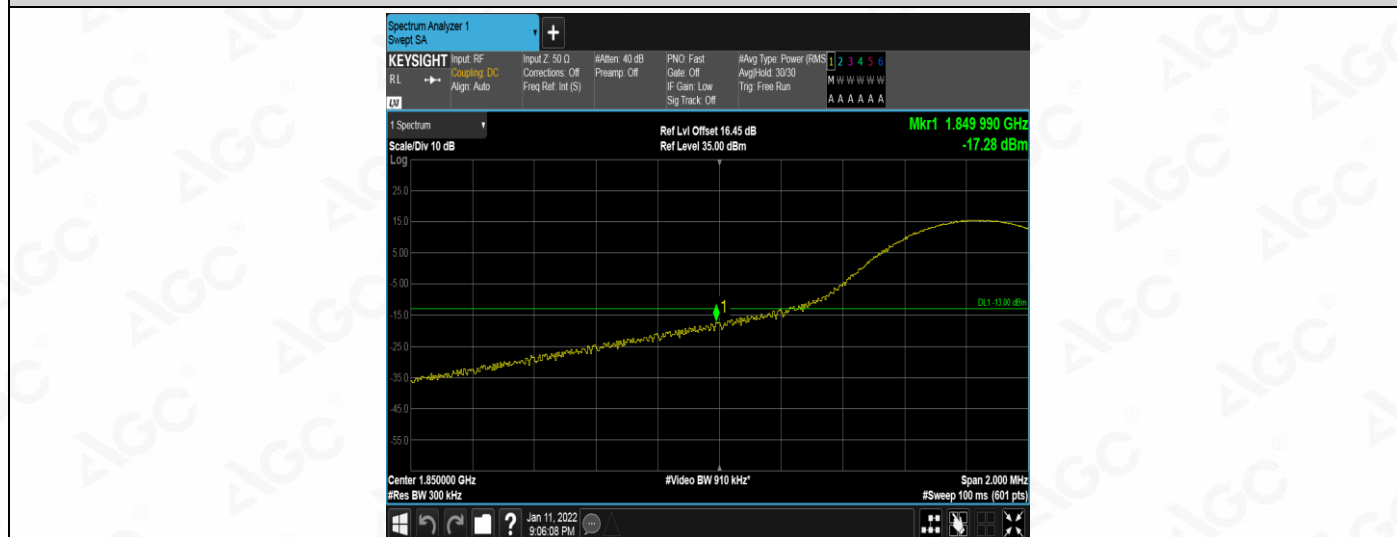
Band25-15MHz-QPSK-26115-1RB#74
