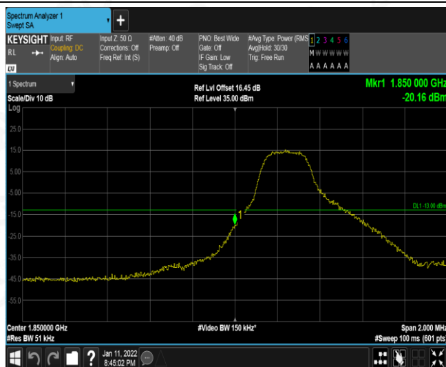
Band25-3MHz-QPSK-26055-1RB#14
