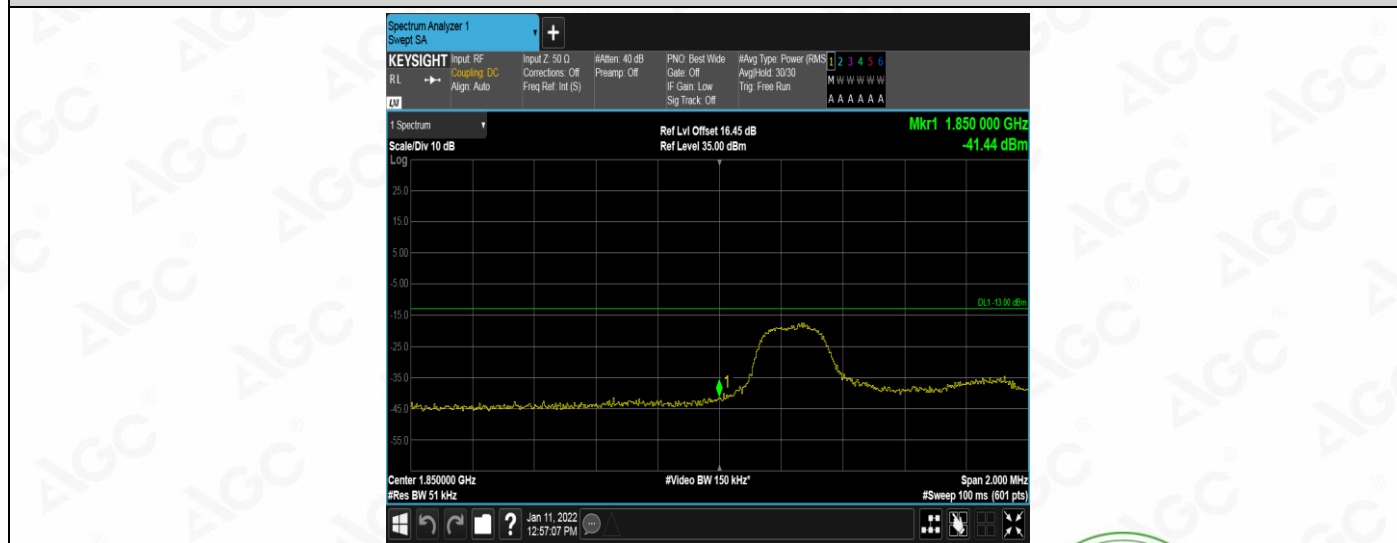
Band25-3MHz-16QAM-26055-1RB#14
