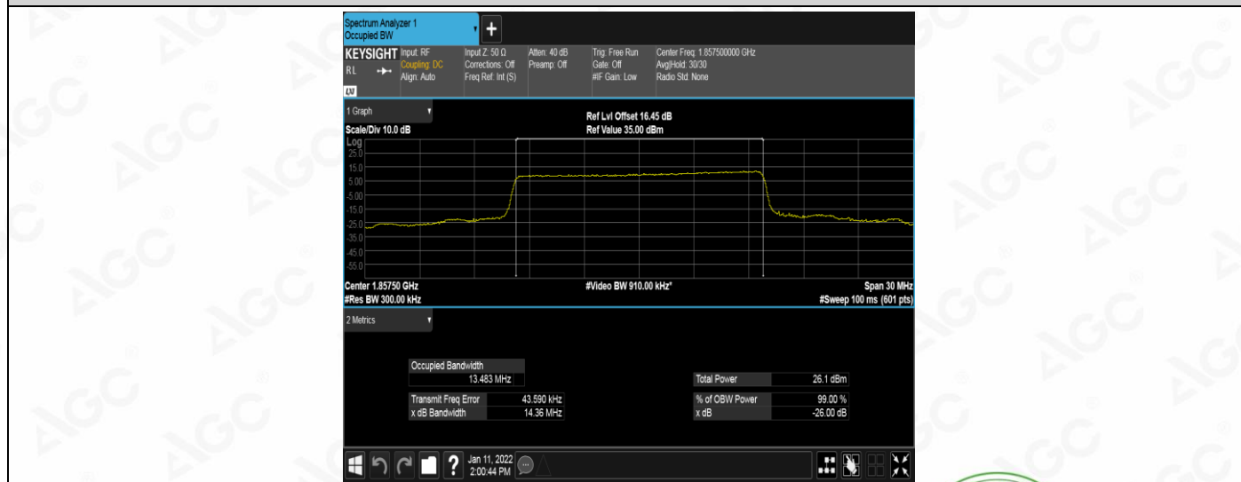
Band25-15MHz-QPSK-26115-75RB#0
