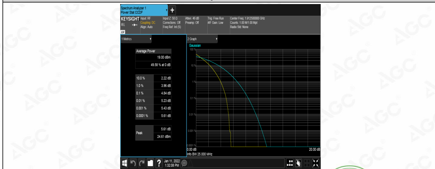
Band25-5MHz-QPSK-26665-25RB#0
