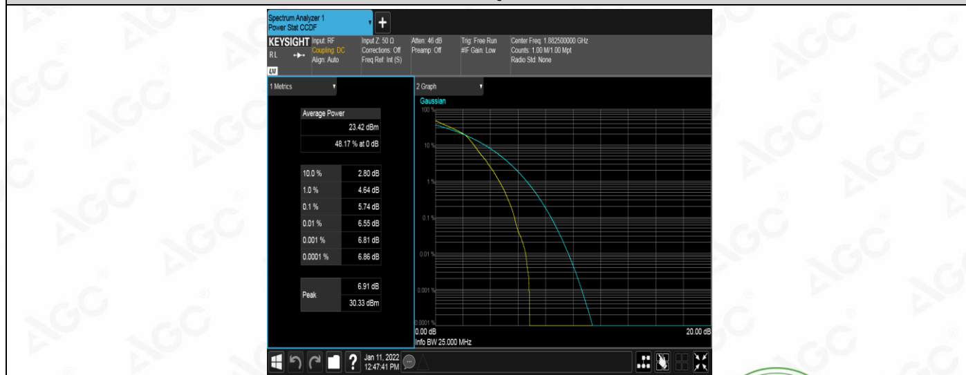
Band25-1.4MHz-16QAM-26365-6RB#0
