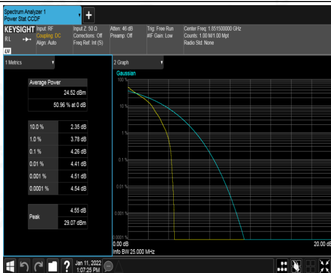
Band25-3MHz-QPSK-26055-15RB#0
