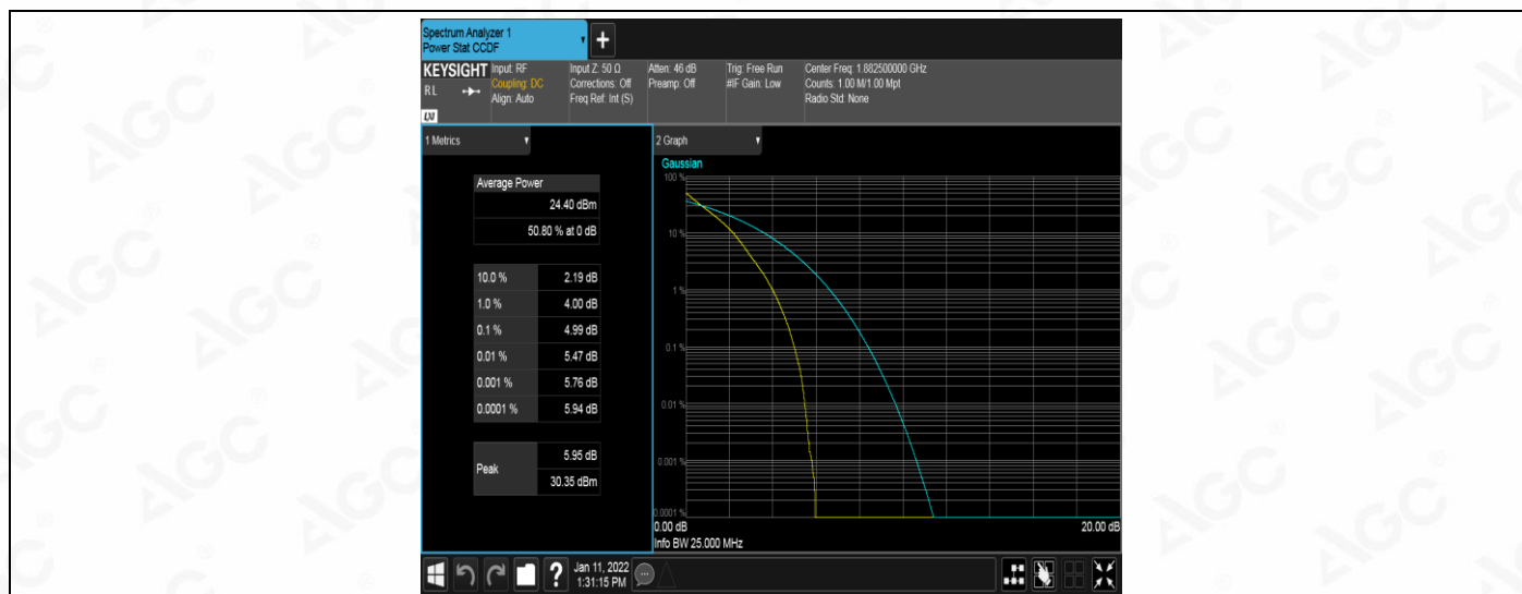
Band25-5MHz-QPSK-26665-1RB#0
