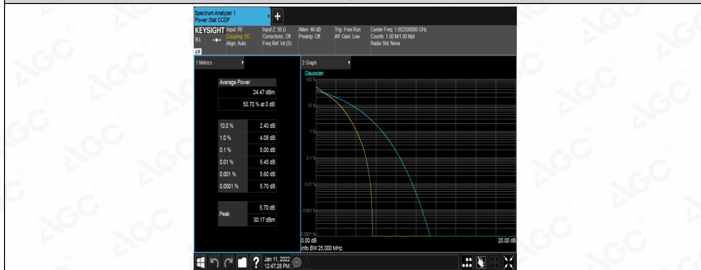
Band25-1.4MHz-QPSK-26683-1RB#0
