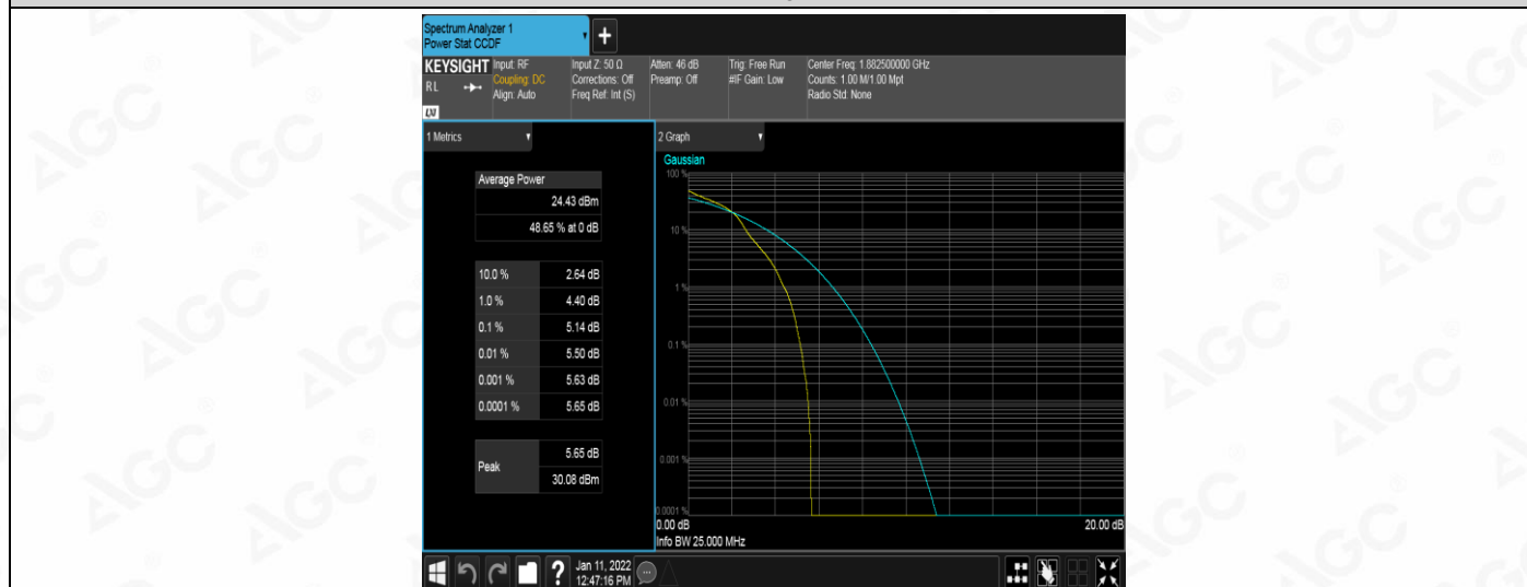
Band25-1.4MHz-16QAM-26365-6RB#0
