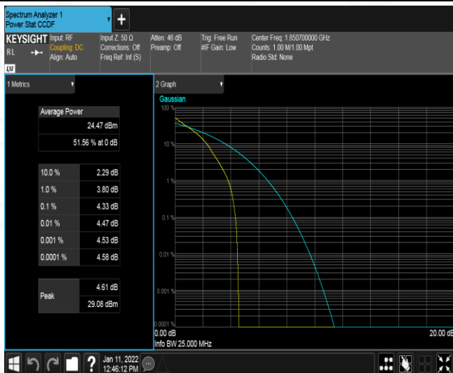
Band25-1.4MHz-QPSK-26047-6RB#0
