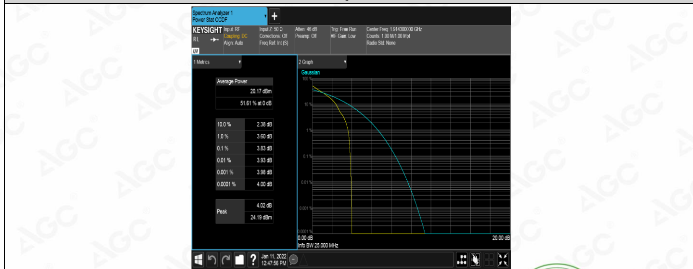
Band25-1.4MHz-QPSK-26683-1RB#0
