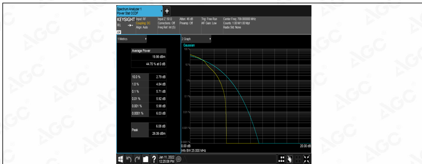
Band13-5MHz-16QAM-23205-25RB#0
