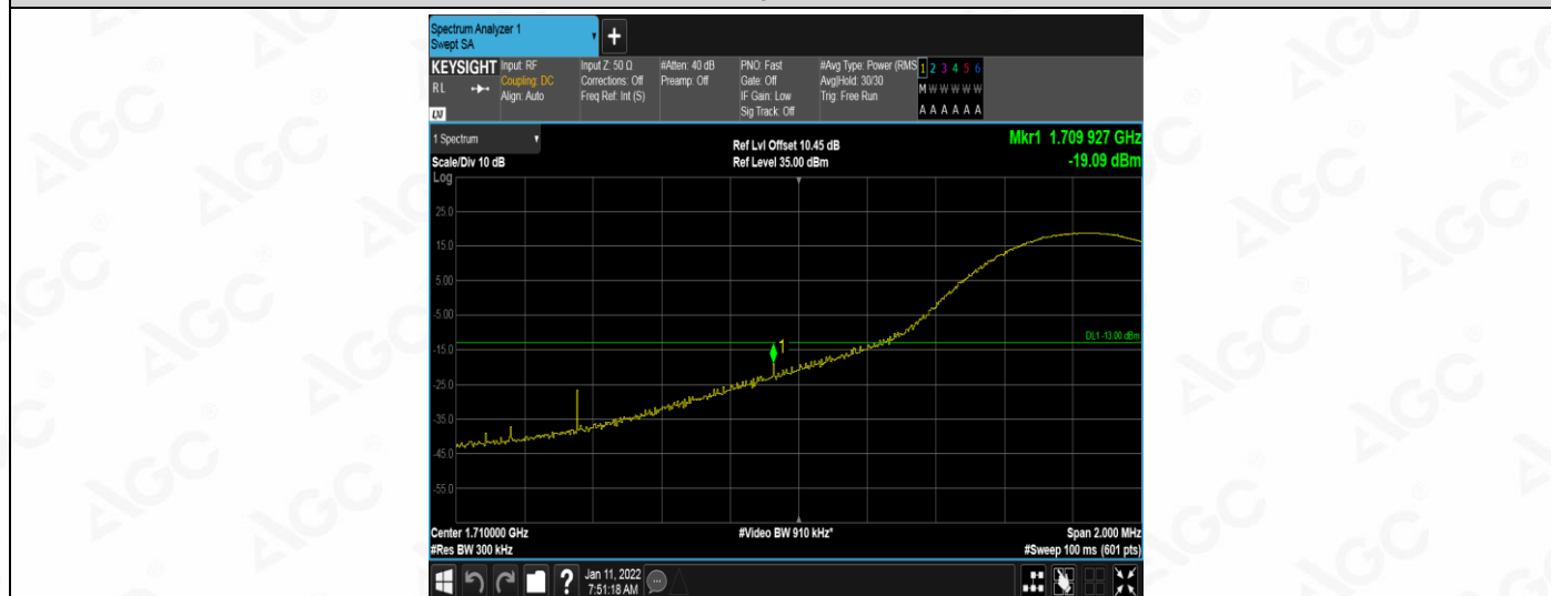
Band4-15MHz-QPSK-20025-1RB#74
