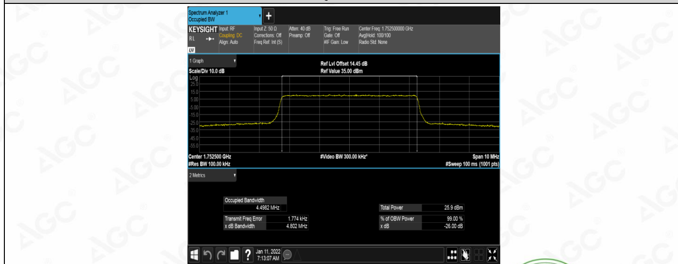
Band4-5MHz-QPSK-20375-25RB#0
