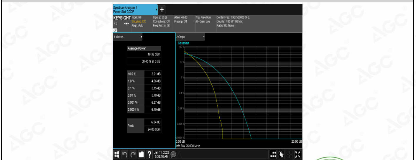
Band2-5MHz-QPSK-19175-25RB#0
