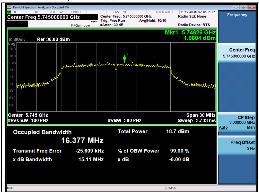
Test_Graph_802.11a_ANT1_5745_6Mbps_DTBSW
