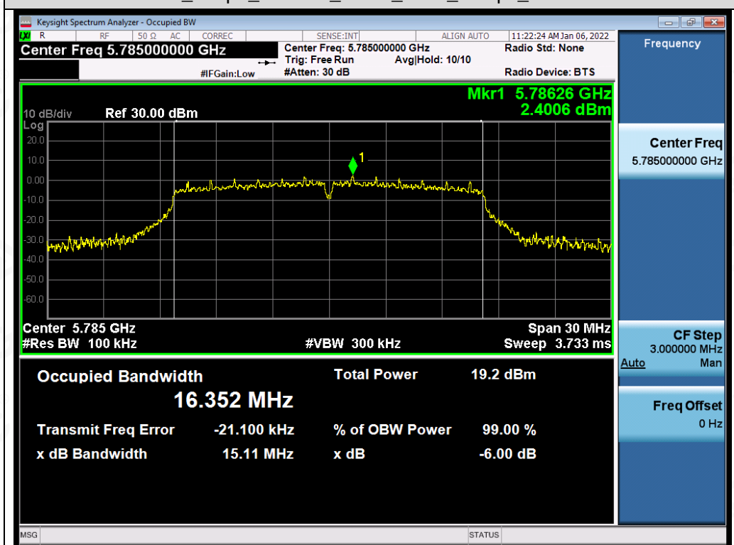
Test_Graph_802.11a_ANT1_5785_6Mbps_DTBSW
