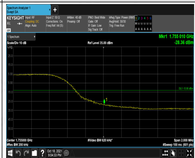
HCH_16QAM_50RB#0
