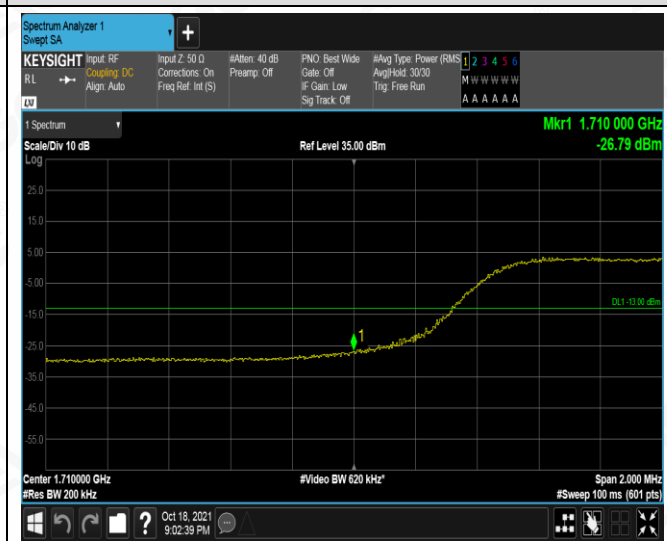
LCH_16QAM_50RB#0
