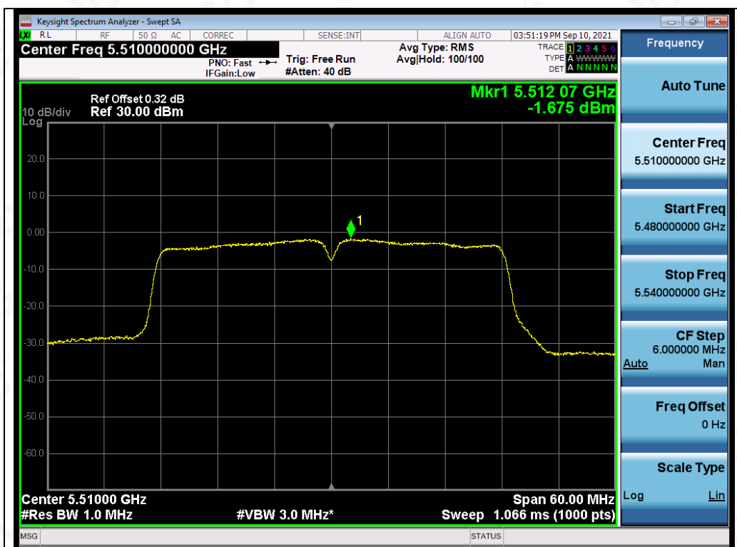
Test_Graph_802.11ac40_ANT2_5510_MCS9_PSD
