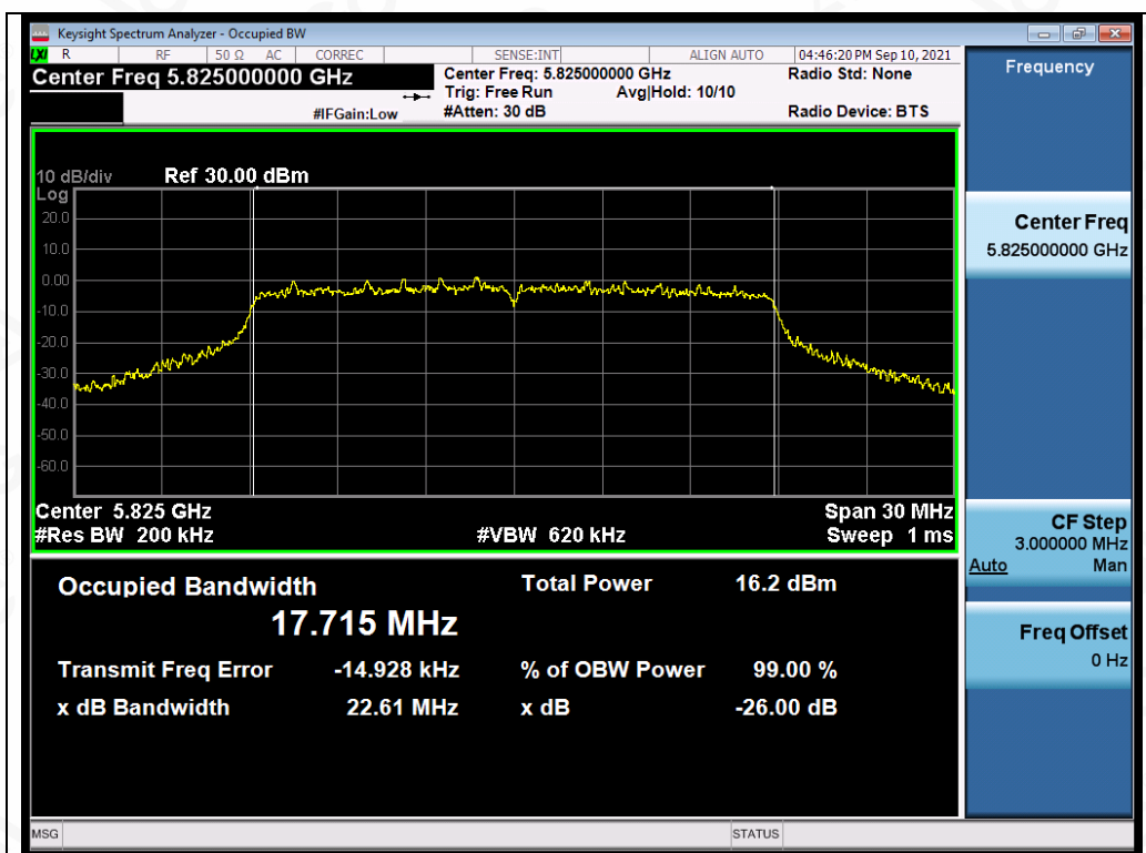
Test_Graph_802.11n20_ANT2_5825_MCS0_OBW
