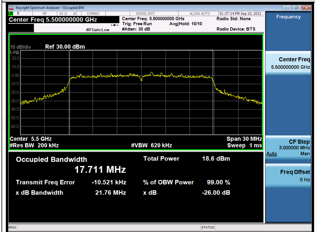
Test_Graph_802.11n20_ANT2_5500_MCS0_OBW
