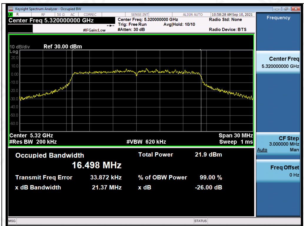
Test_Graph_802.11a_ANT2_5320_6Mbps_OBW
