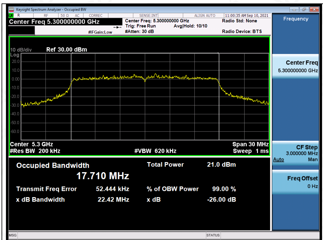
Test_Graph_802.11n20_ANT2_5300_MCS0_OBW
