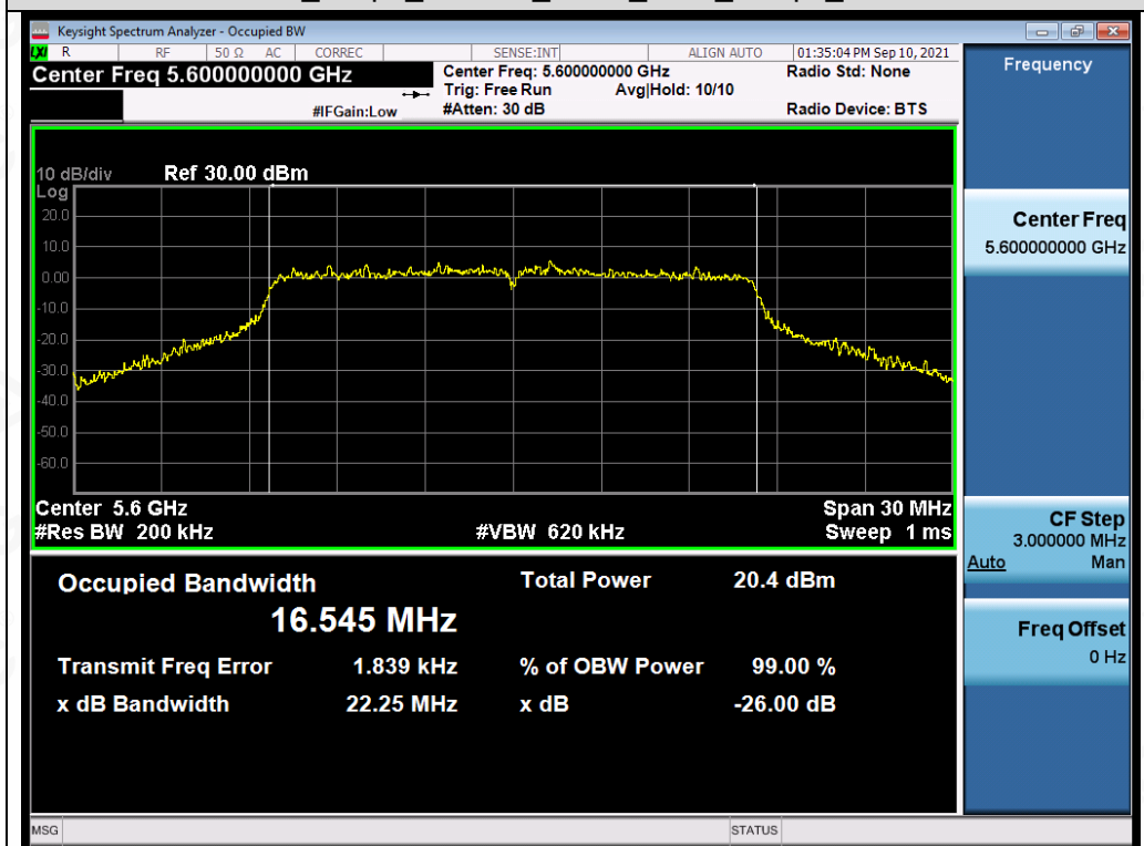
Test_Graph_802.11a_ANT2_5600_6Mbps_OBW
