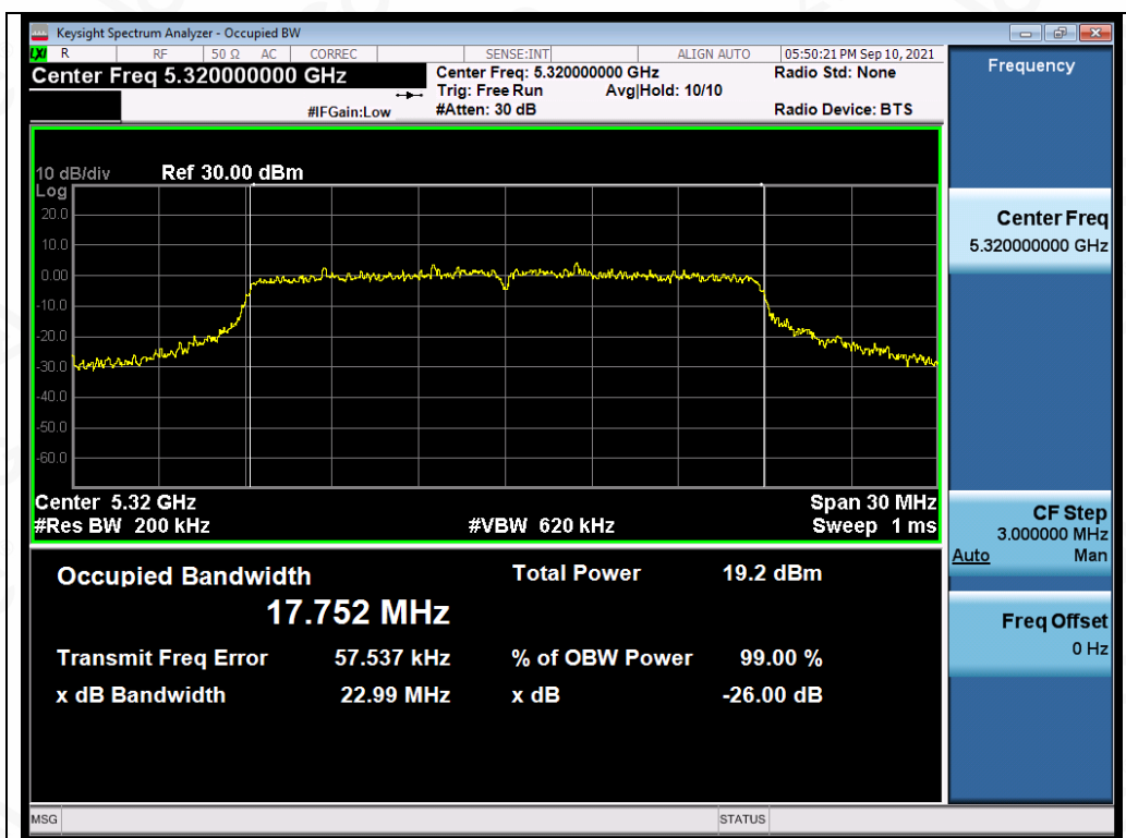
Test_Graph_802.11ac20_ANT2_5320_MCS9_OBW
