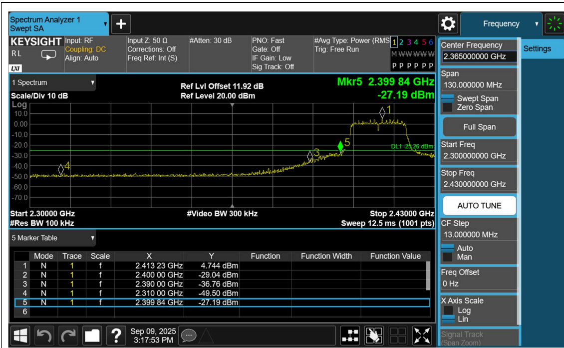
11N20SISO_Ant1_Low_2412
