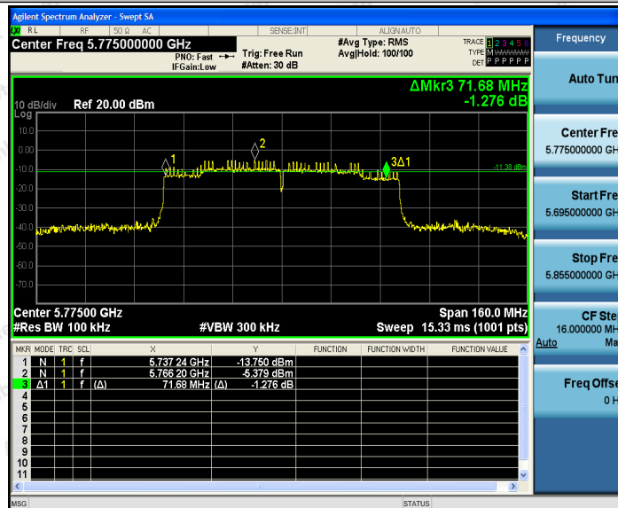
11AC80SISO_Ant2_5775
