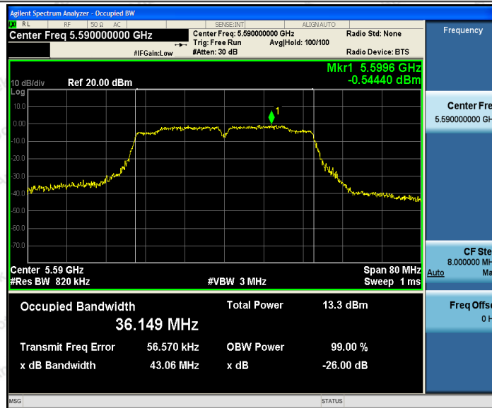
11AC40SISO_Ant2_5590
