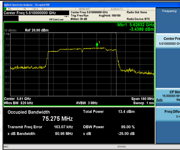
11AC80SISO_Ant2_5610
