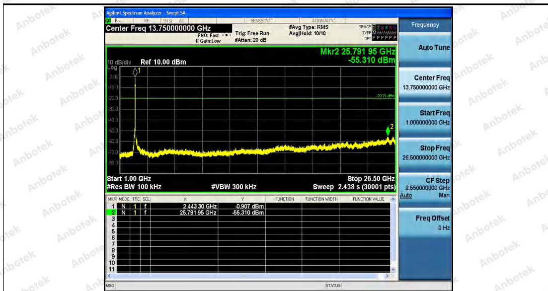
11N40_Ant2_2437_0~Reference
