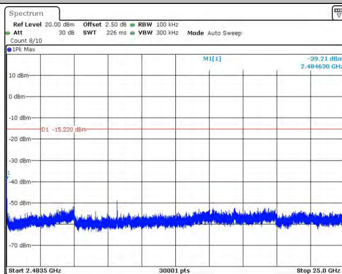
11N20_Ant1_2462_2483.5~25000
