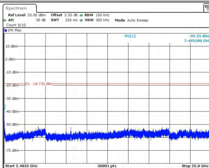
11N40_Ant1_2437_2483.5~25000
