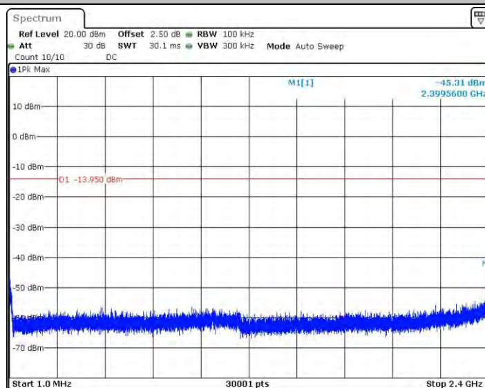
11N20_Ant2_2437_1~2400
