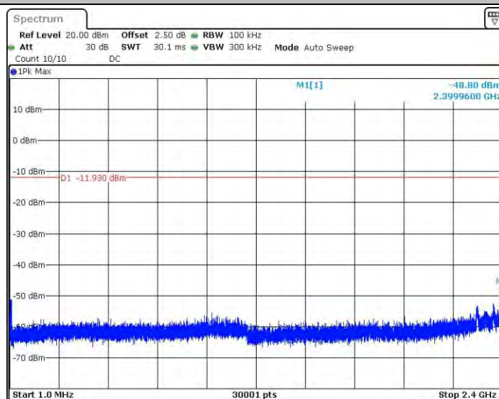
11B_Ant1_2437_1~2400
