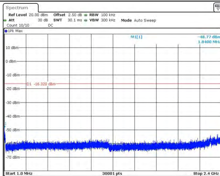
11G_Ant1_2437_1~2400
