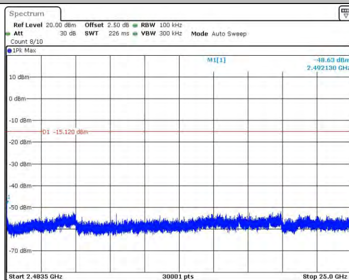
11N20_Ant1_2412_2483.5~25000
