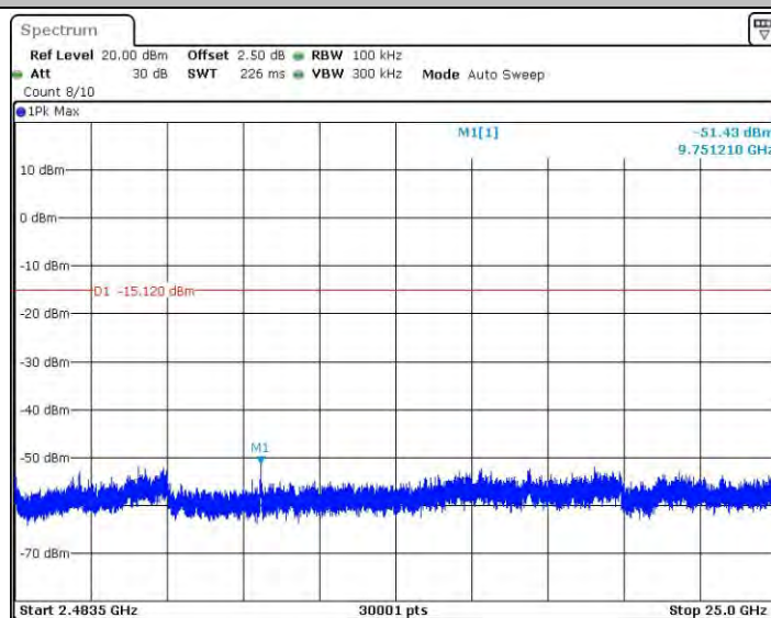
11N20_Ant1_2437_2483.5~25000
