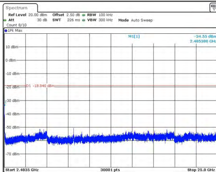
11N40_Ant1_2452_2483.5~25000
