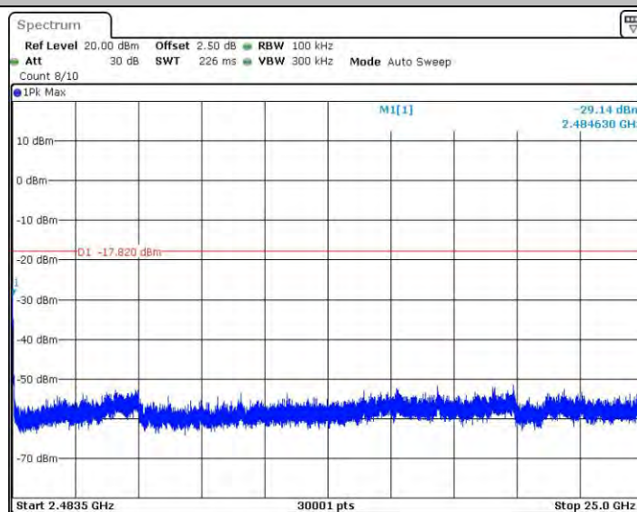
11N40_Ant2_2452_2483.5~25000
