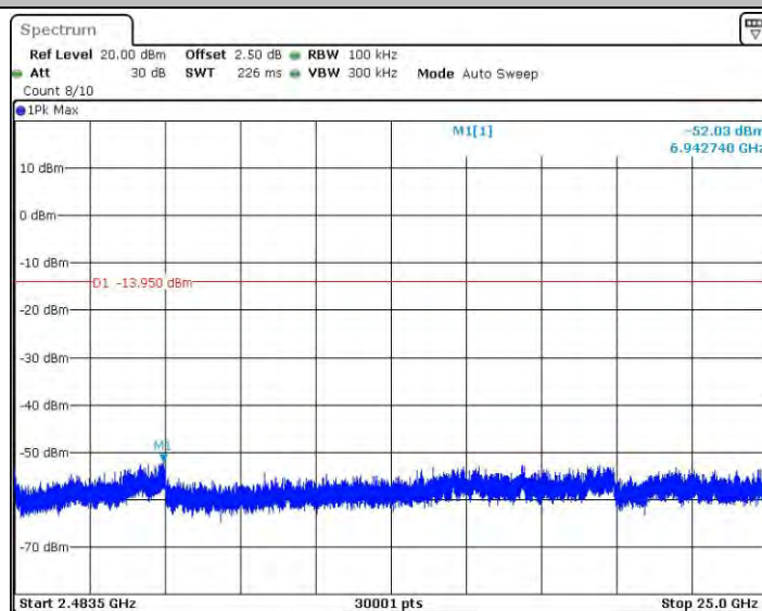
11N20_Ant2_2437_2483.5~25000
