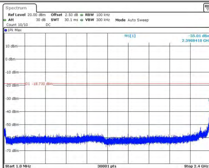
11N40_Ant1_2437_1~2400
