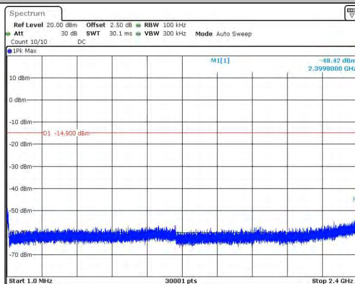
11G_Ant2_2437_1~2400
