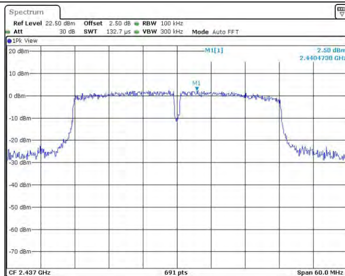
11N40_Ant2_2437_0~Reference
