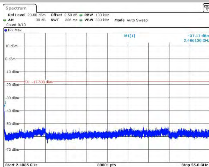
11N40_Ant2_2437_2483.5~25000
