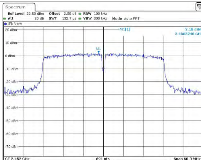
11N40_Ant2_2452_0~Reference
