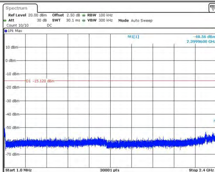
11N20_Ant1_2437_1~2400
