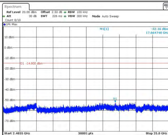
11G_Ant2_2437_2483.5~25000
