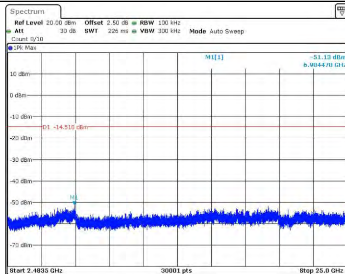
11N20_Ant2_2412_2483.5~25000
