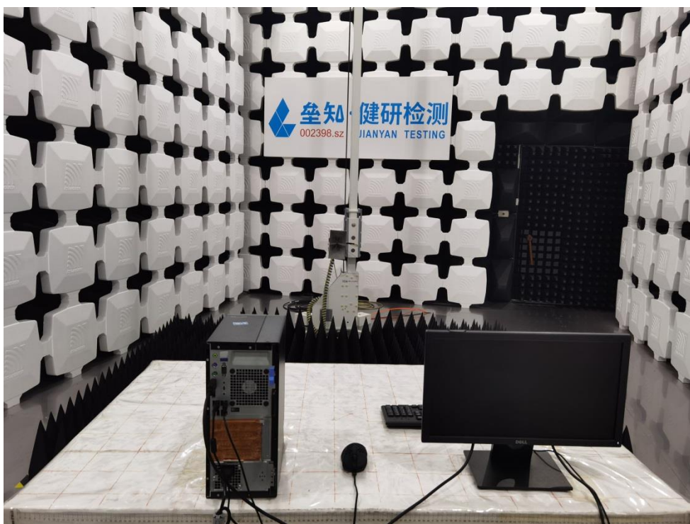
Above 1GHz
