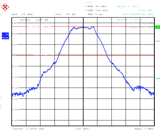
26dB&99% Occupied Bandwidth Plot on Channel 512
