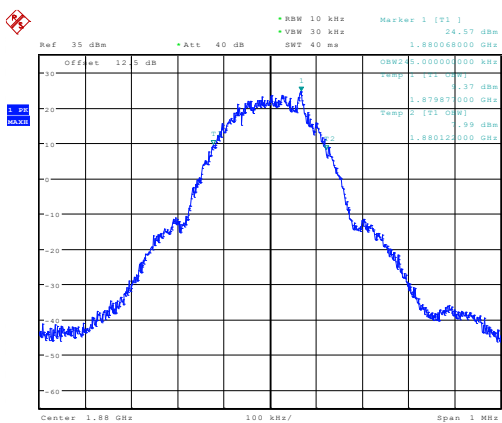
26dB&99% Occupied Bandwidth Plot on Channel 661
