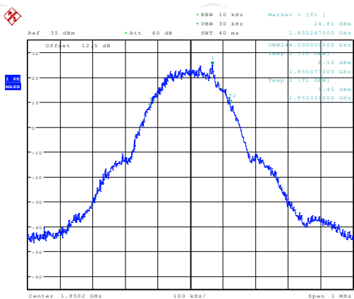
26dB&99% Occupied Bandwidth Plot on Channel 512
