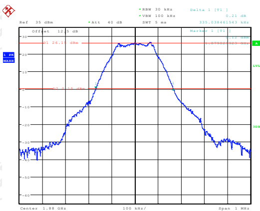
26dB&99% Occupied Bandwidth Plot on Channel 661
