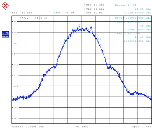
26dB&99% Occupied Bandwidth Plot on Channel 810
