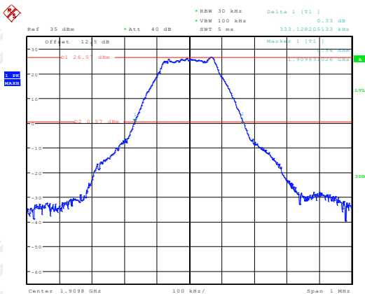
26dB&99% Occupied Bandwidth Plot on Channel 810
