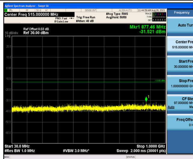
Band2-15MHz-16QAM-18675-1RB#0-Range4:1000~5000MHz
