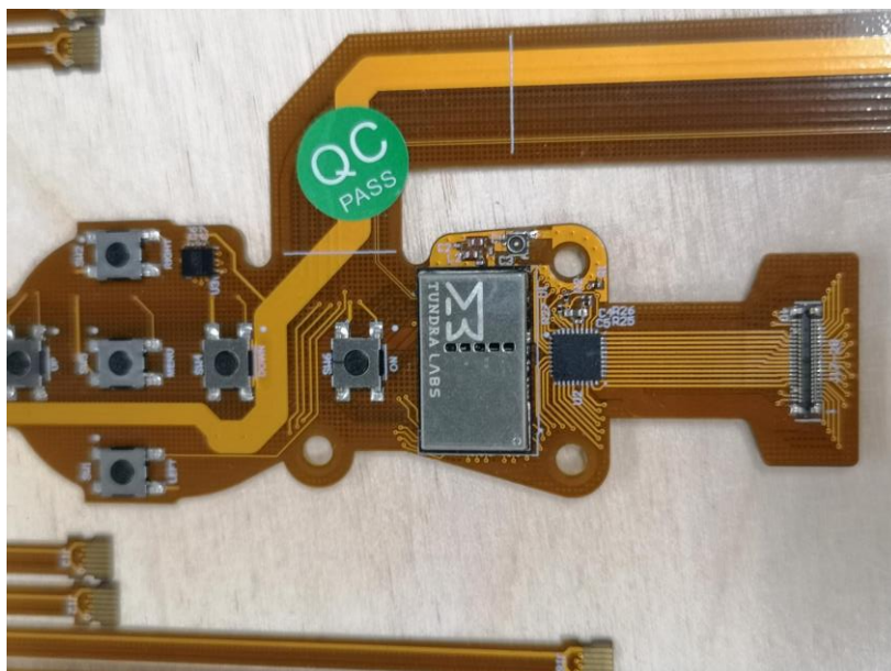
Radio module and MH4 UFL
