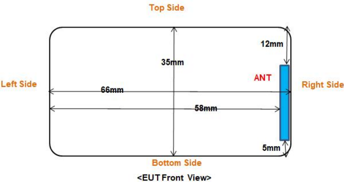
Fig 7.1 Block Diagram for EUT Antenna Position EUT Size: Long*Width*Height=66mm*35mm*20mm
